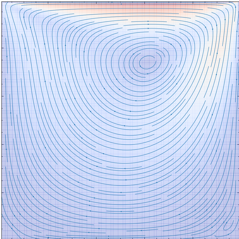
Streamlines — Simulation ID: 4f586c7b
