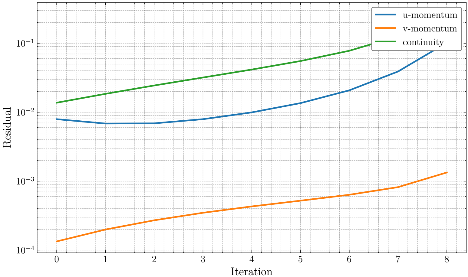
Residual History — Simulation ID: c14e94f9
