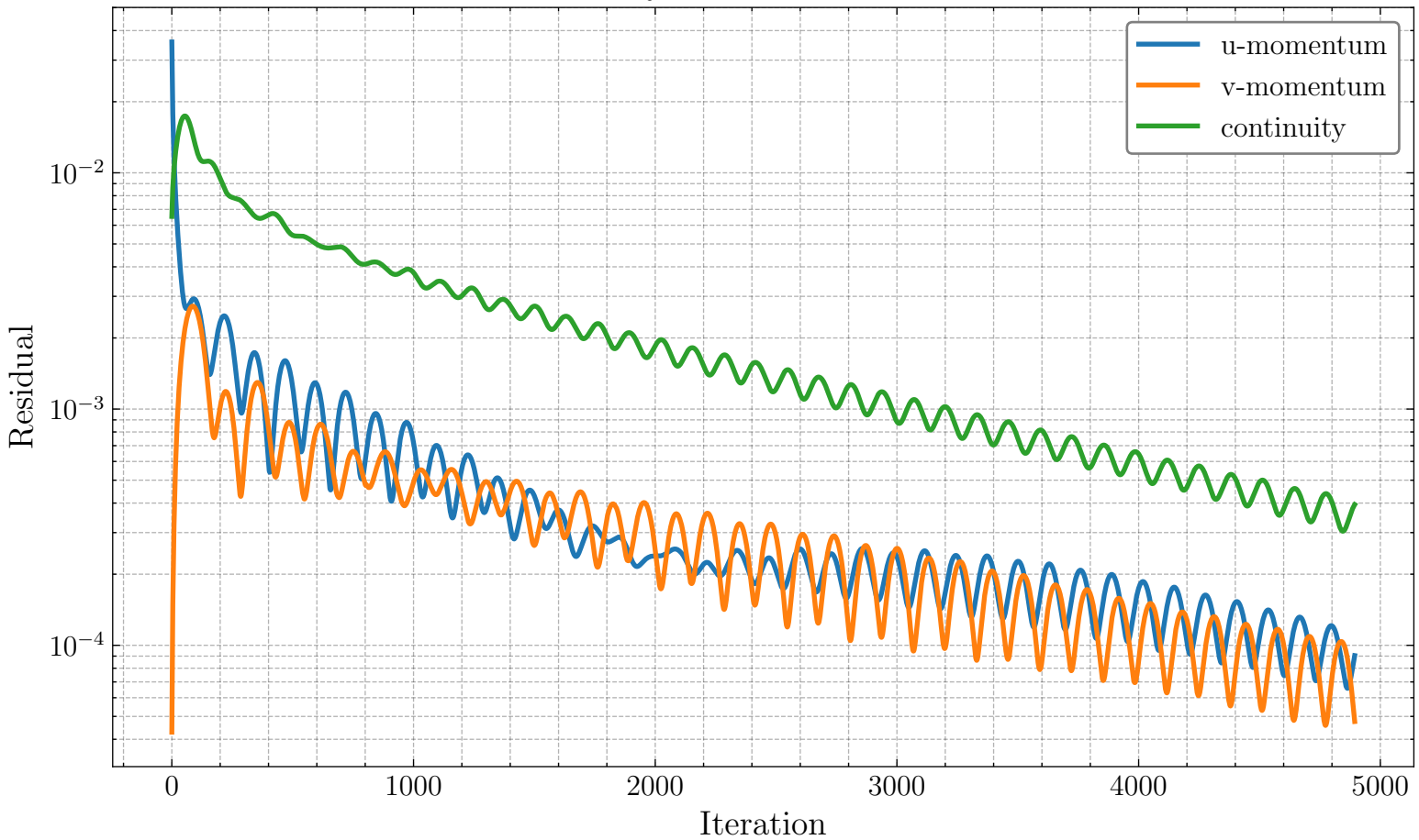
Residual History — Simulation ID: 5e7591a2
