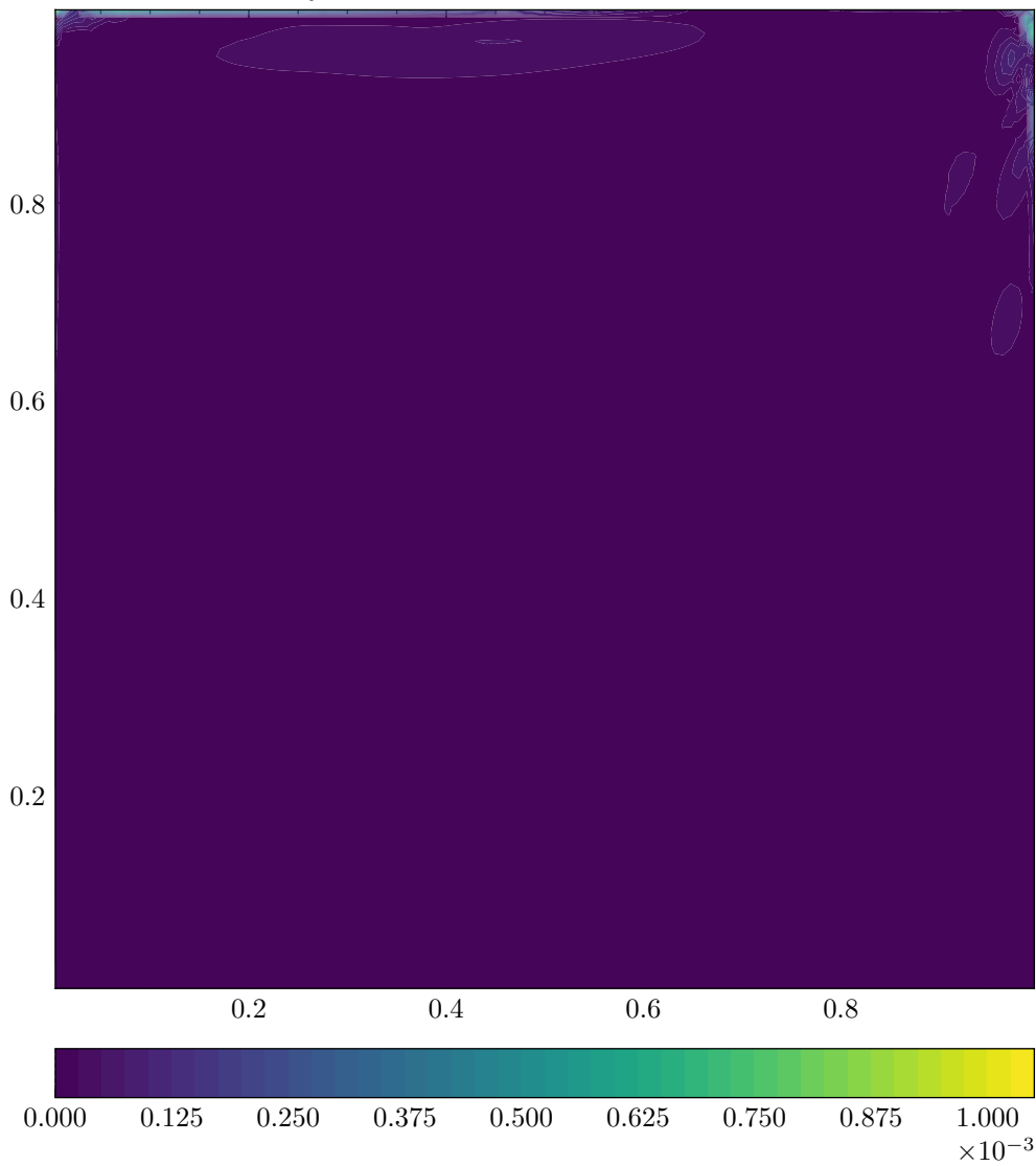
Continuity Residual — Simulation ID: 2e7f0f18
