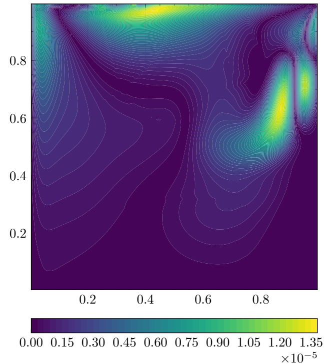
V Residual
