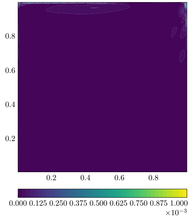
Continuity Residual
