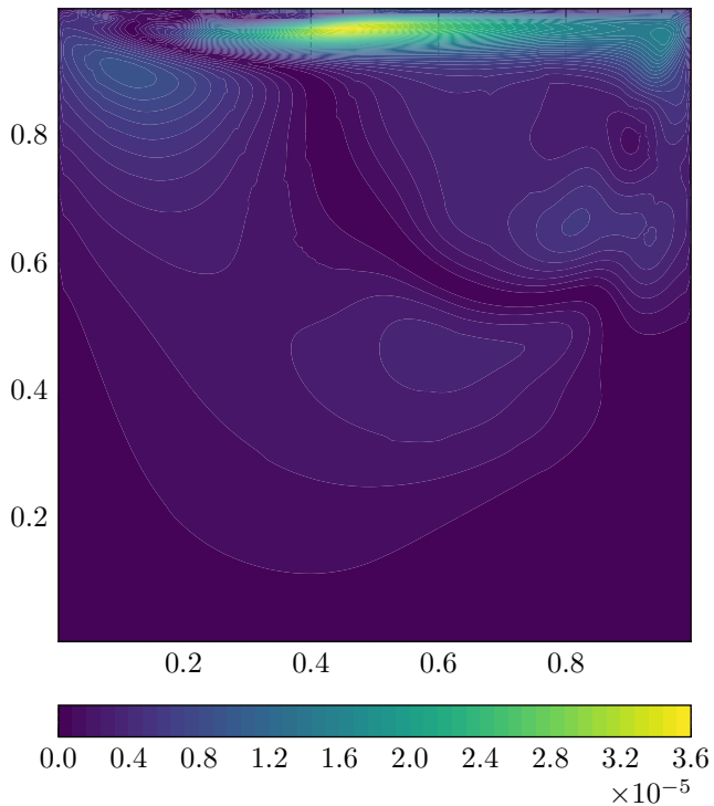
U Residual
