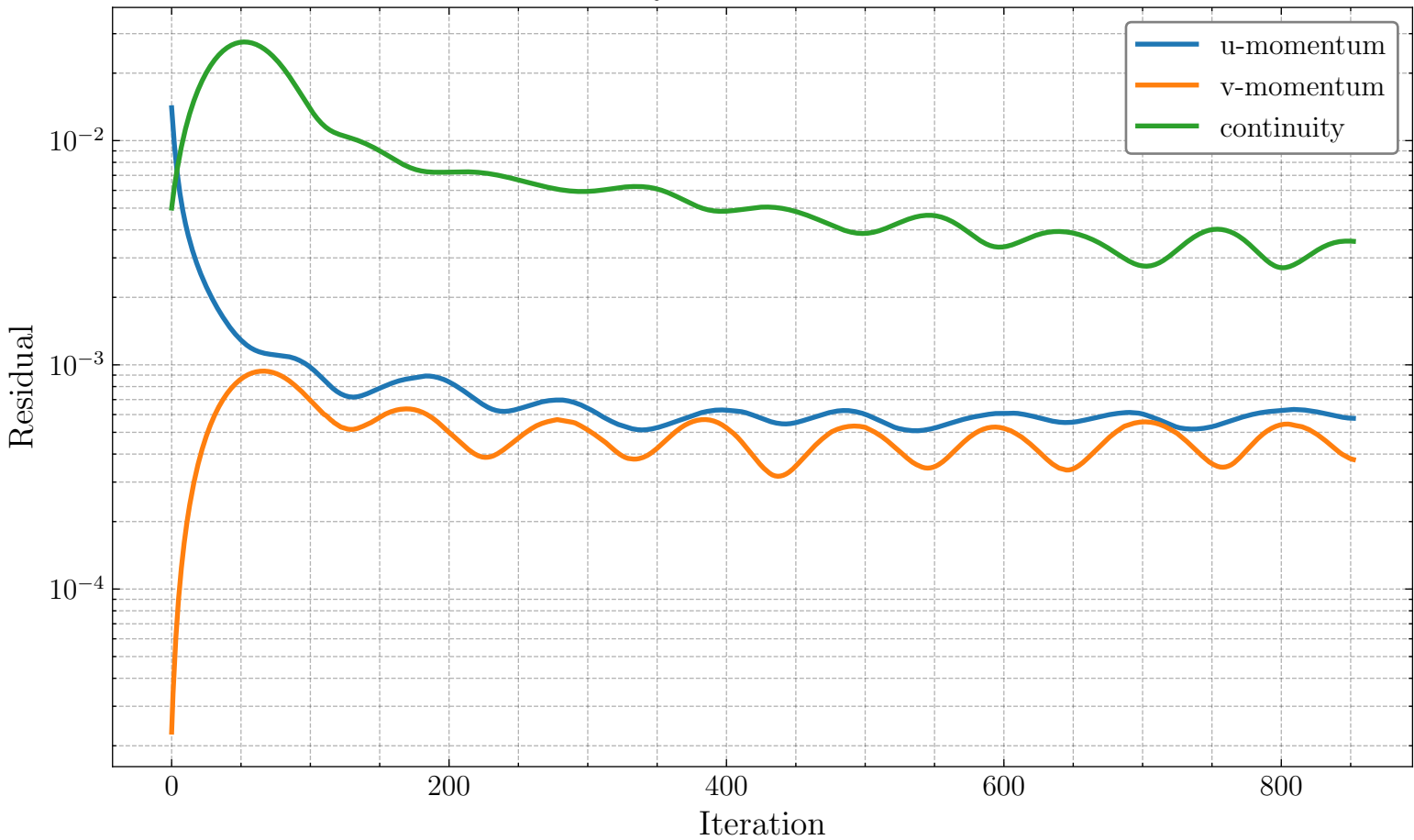
Residual History — Simulation ID: 2e7f0f18
