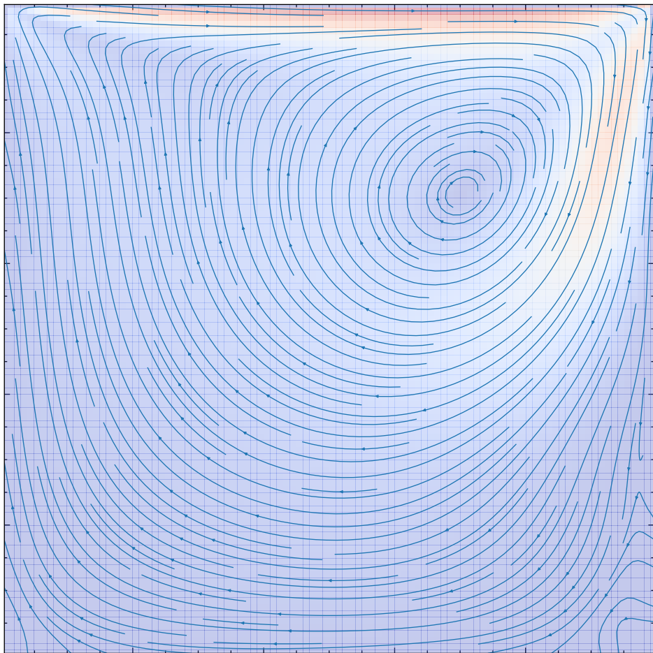
Streamlines — Simulation ID: 2e7f0f18
