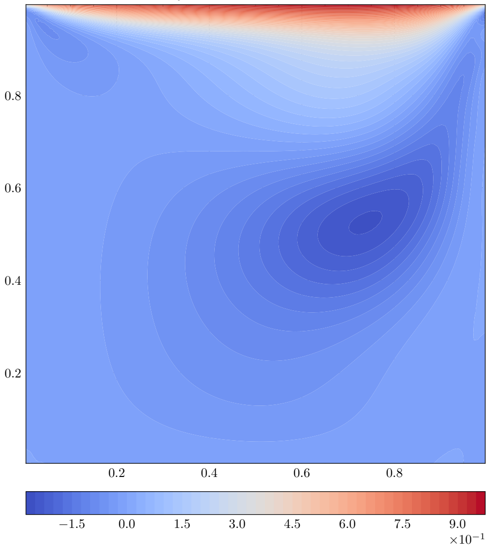
u-velocity — Simulation ID: 2e7f0f18
