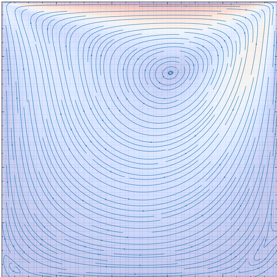
Streamlines — Simulation ID: 2c1bb45e
