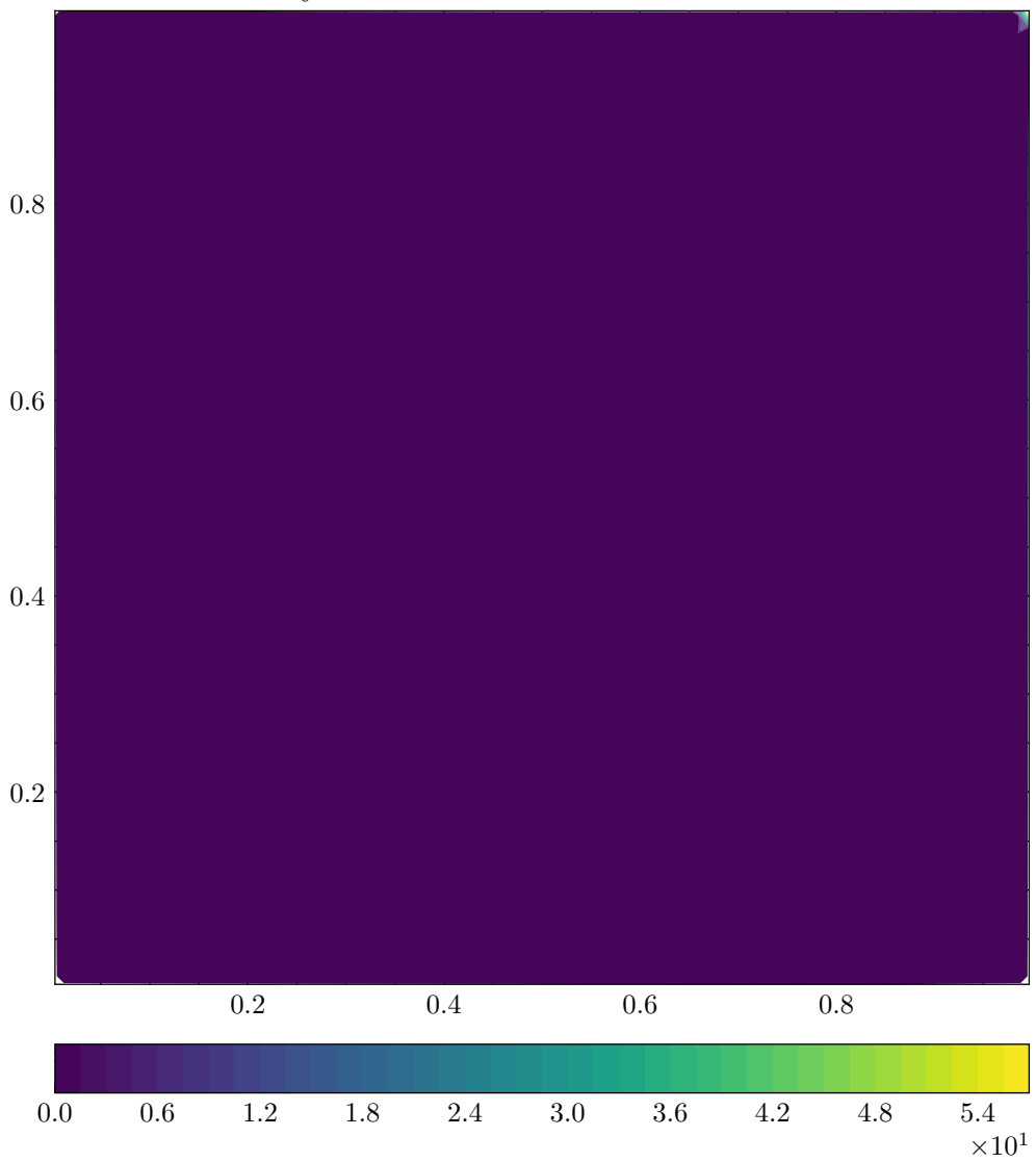
Continuity Residual — Simulation ID: c54600fd
