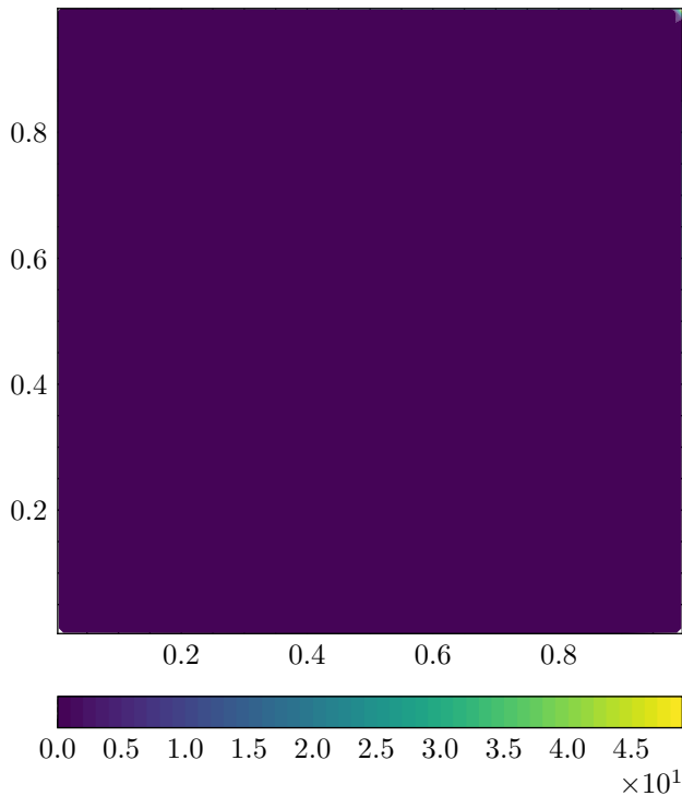
U Residual
