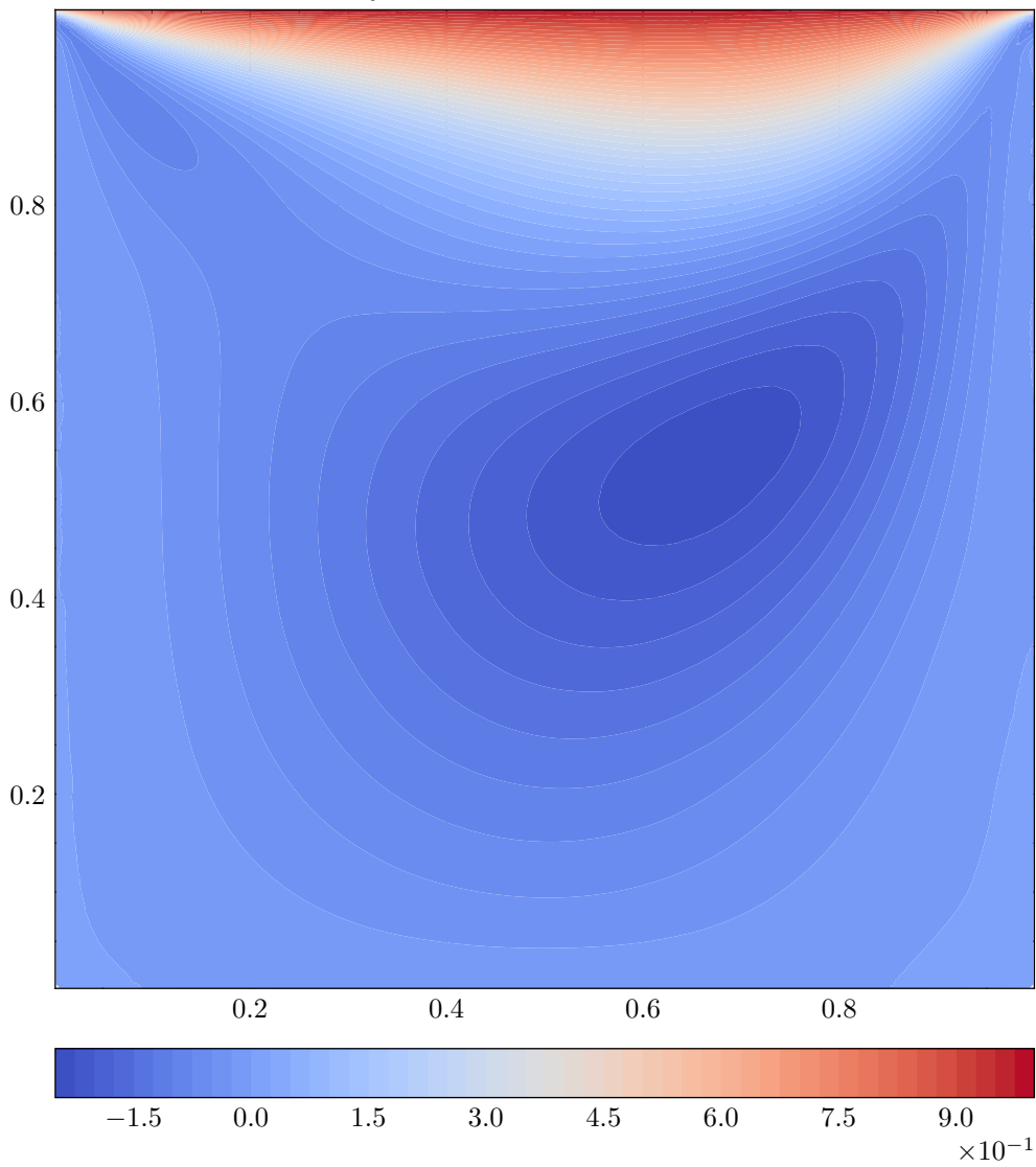
u-velocity — Simulation ID: a0579211
