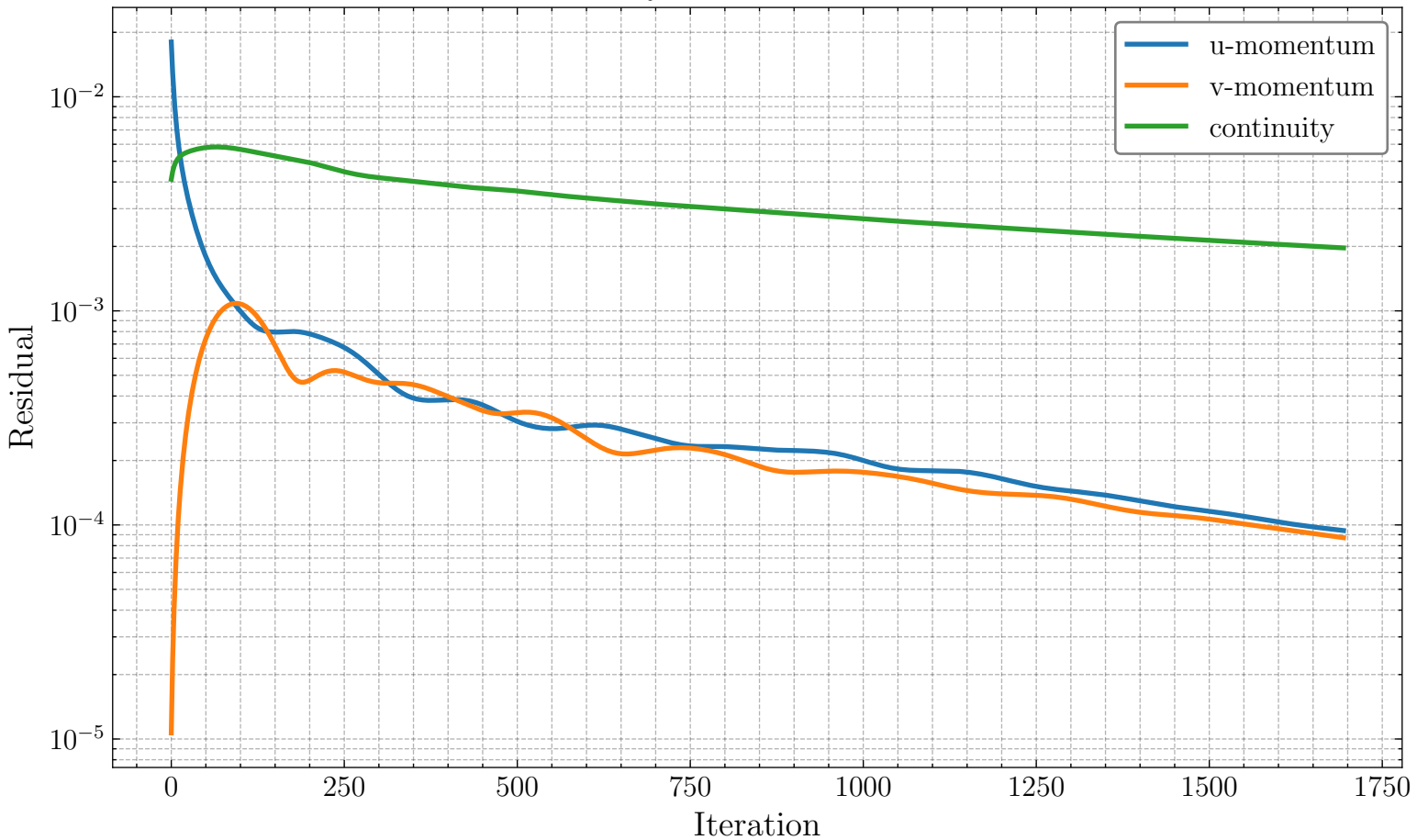
Residual History — Simulation ID: 7f42489f
