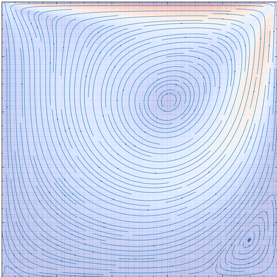
Streamlines — Simulation ID: 7f42489f
