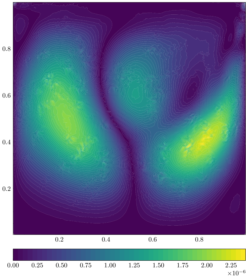
V Residual — Simulation ID: 7f42489f
