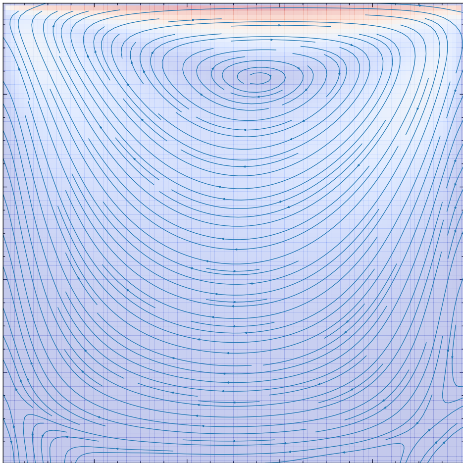
Streamlines — Simulation ID: 9193d6d8
