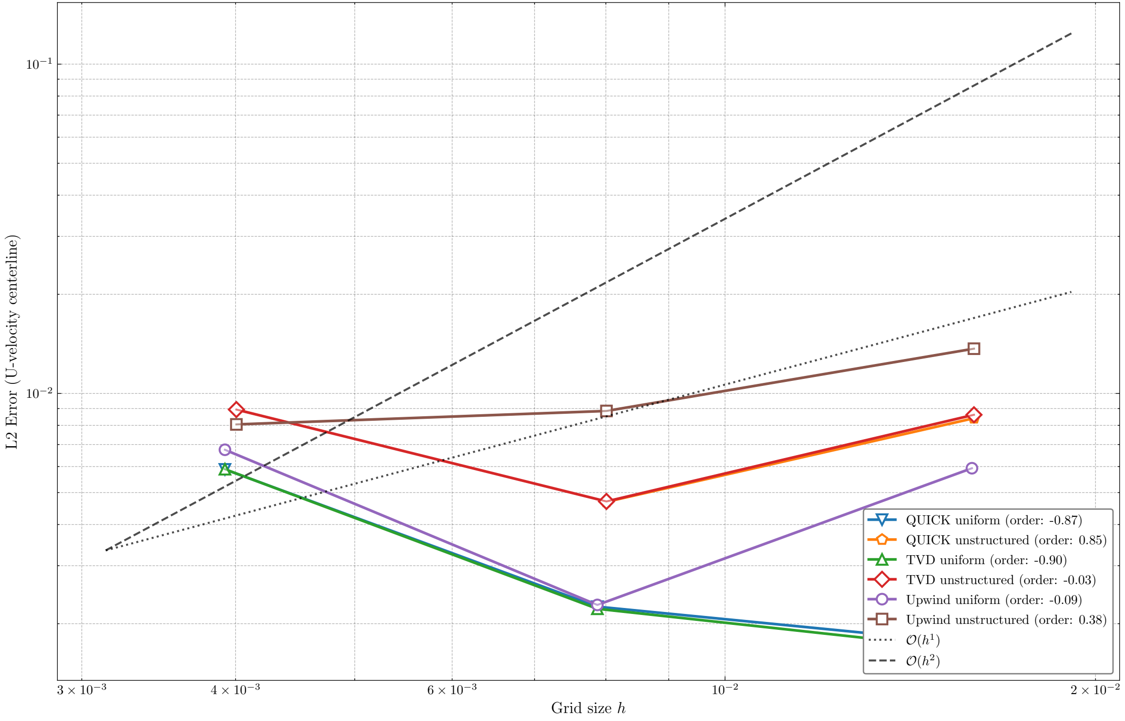
Grid Convergence Study - Re=100
