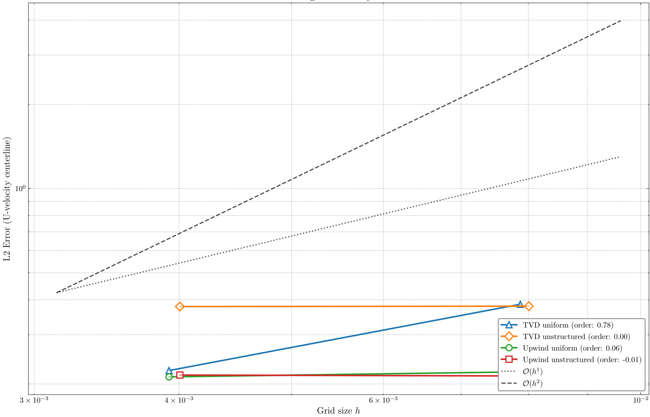
Grid Convergence Study - Re=3200
