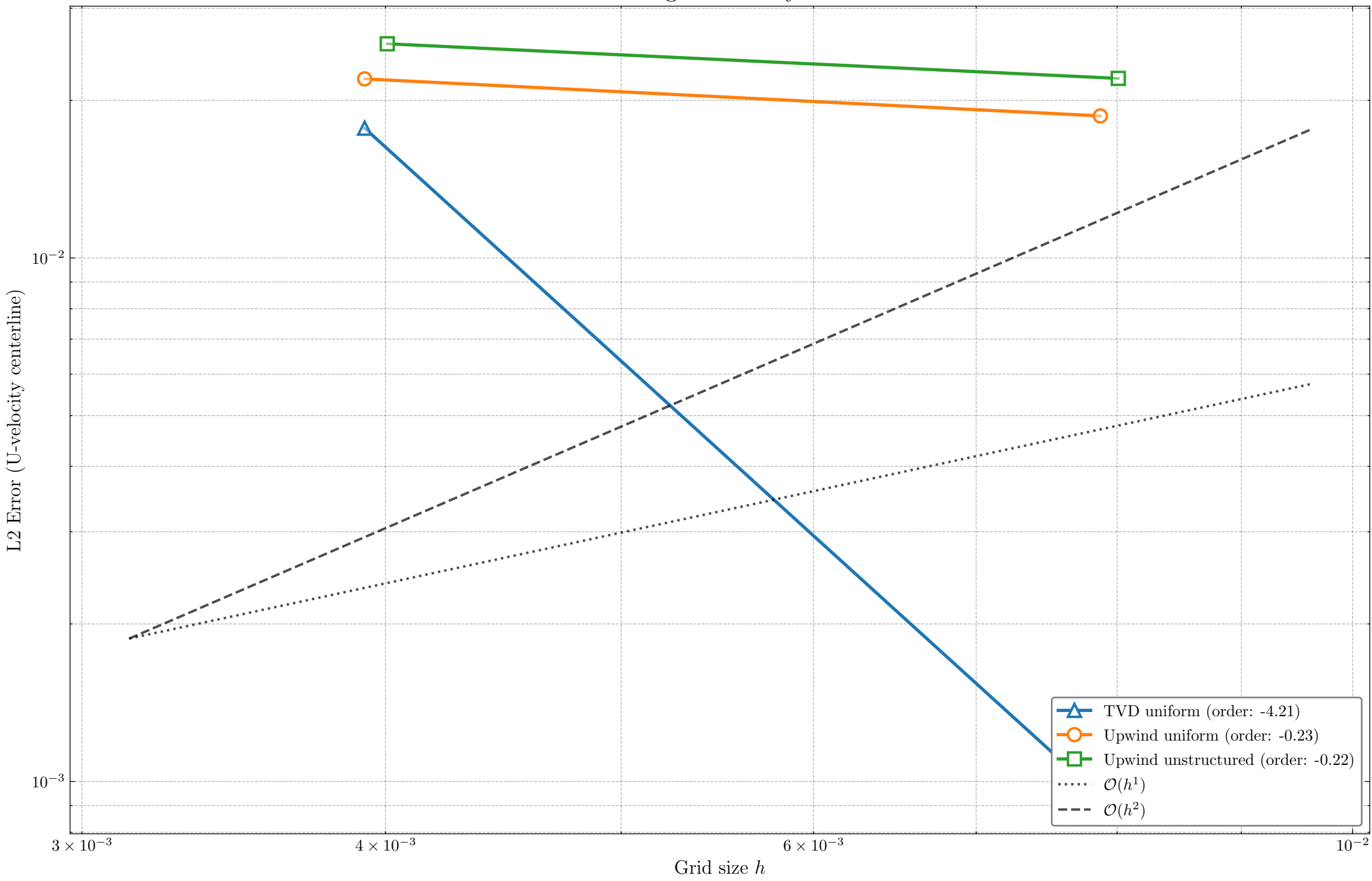
Grid Convergence Study - Re=400
