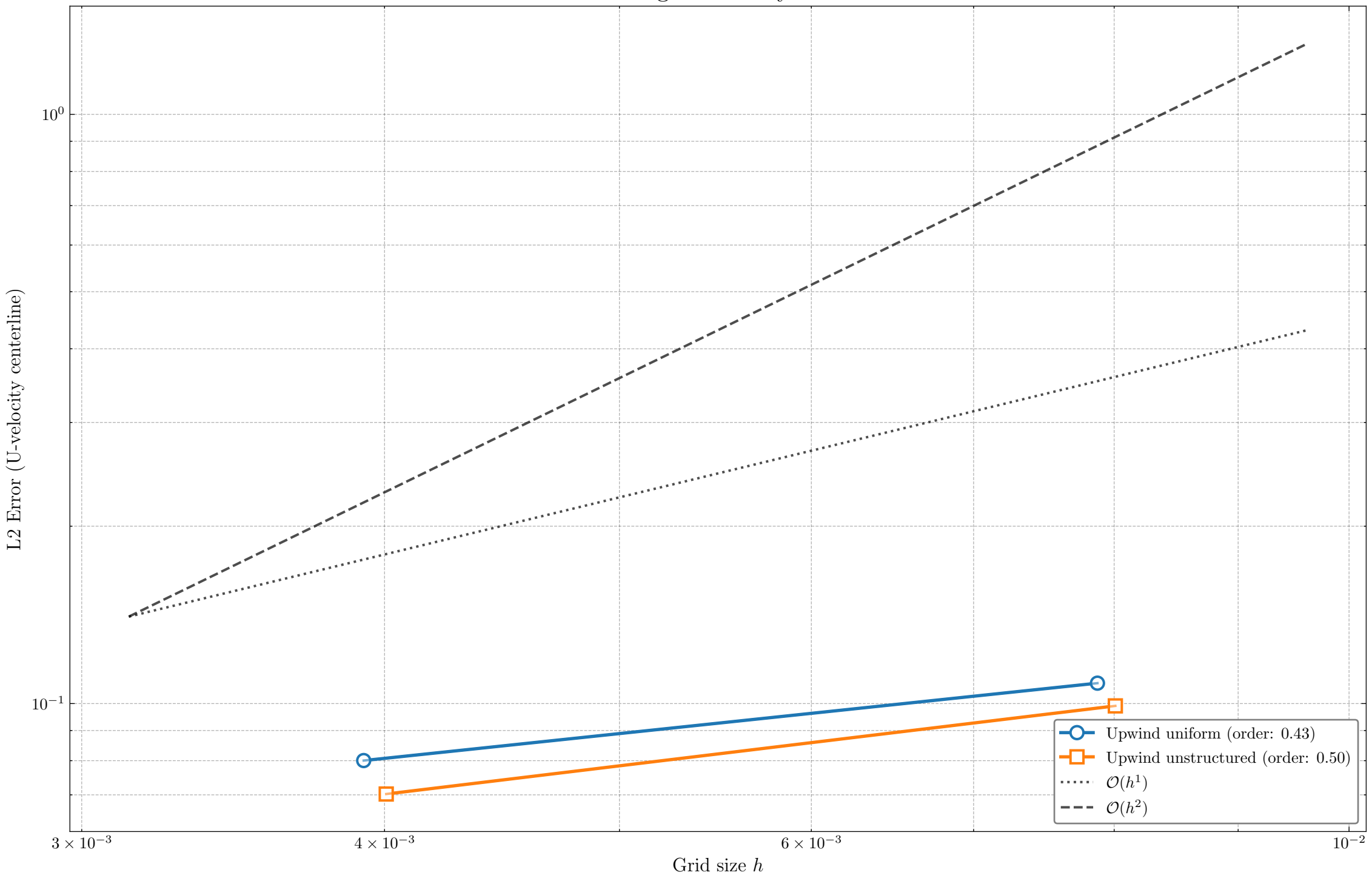
Grid Convergence Study - Re=5000
