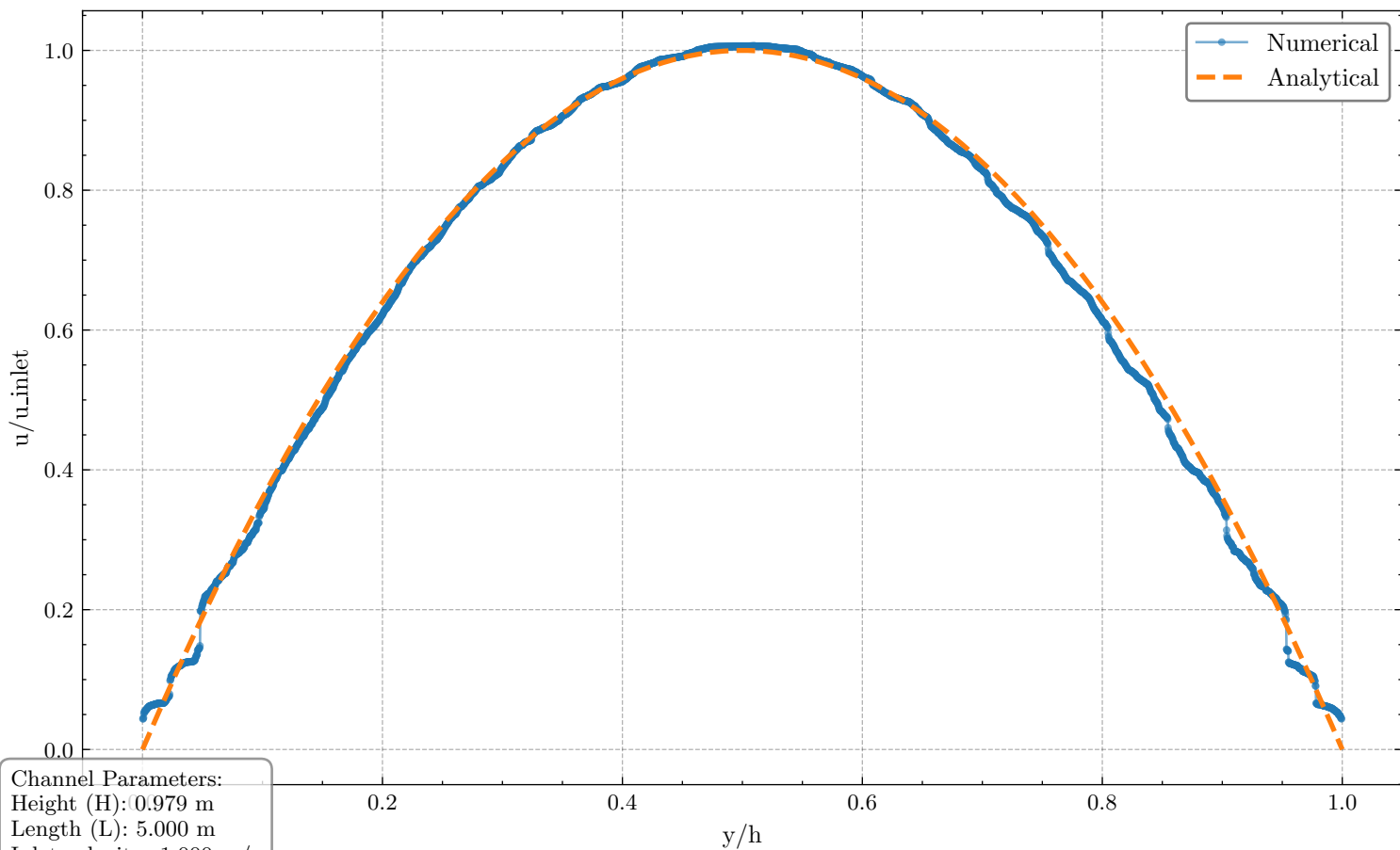
Velocity Profile at x=L/2
