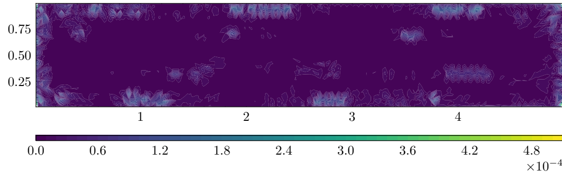
Continuity Residual
