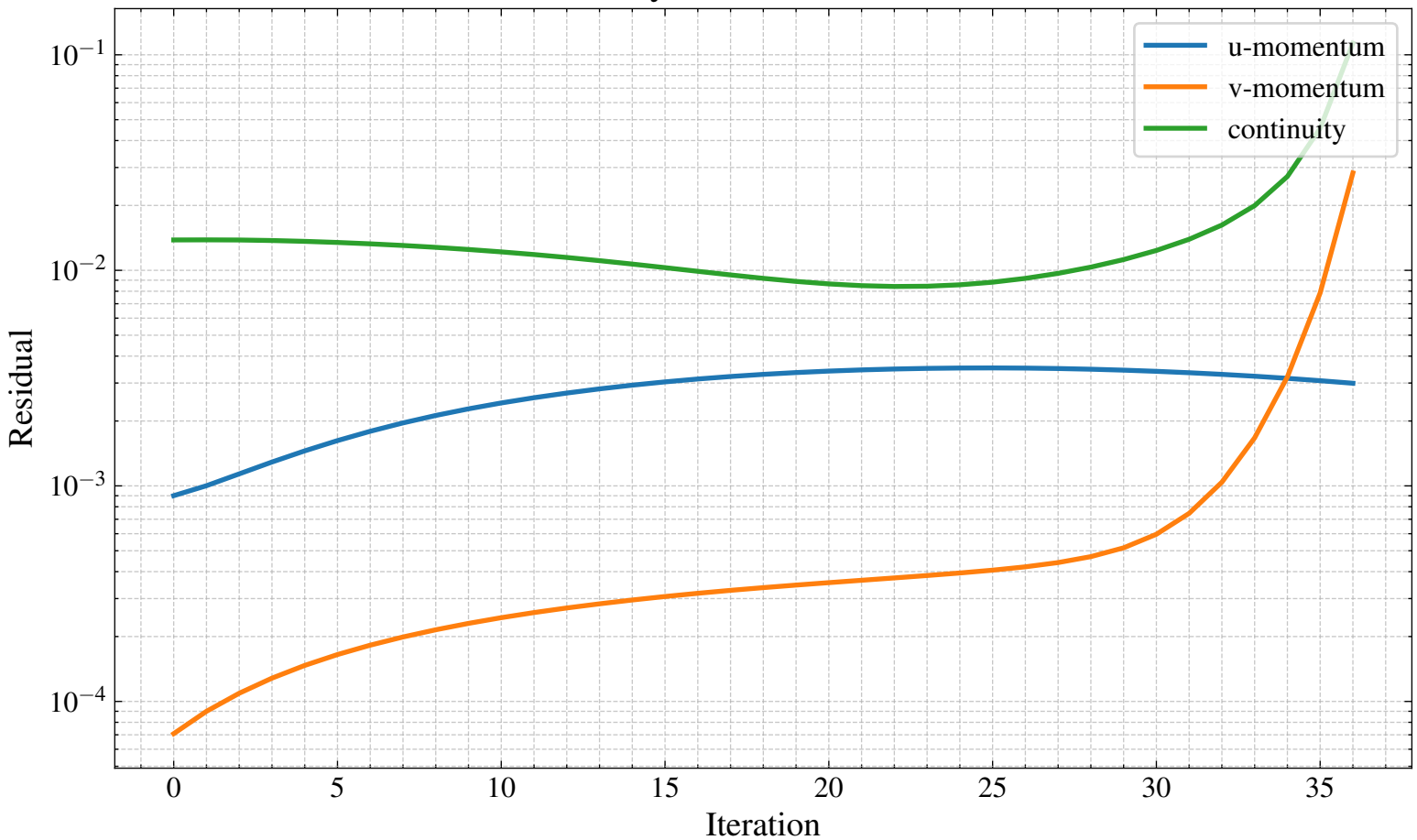
Residual History — Simulation ID: 0a9cde15
