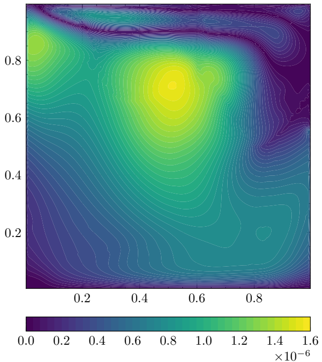
U Residual
