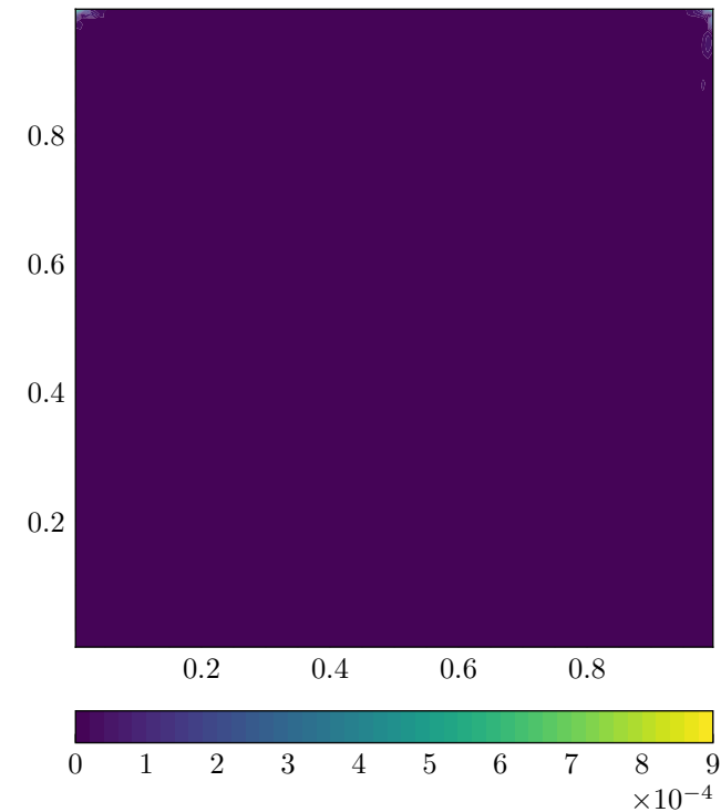
Continuity Residual
