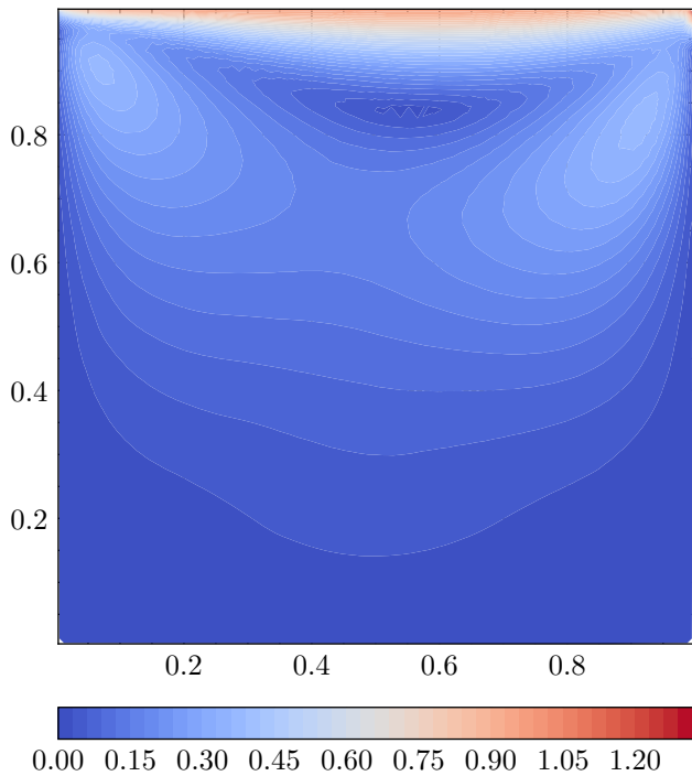
Velocity Magnitude
