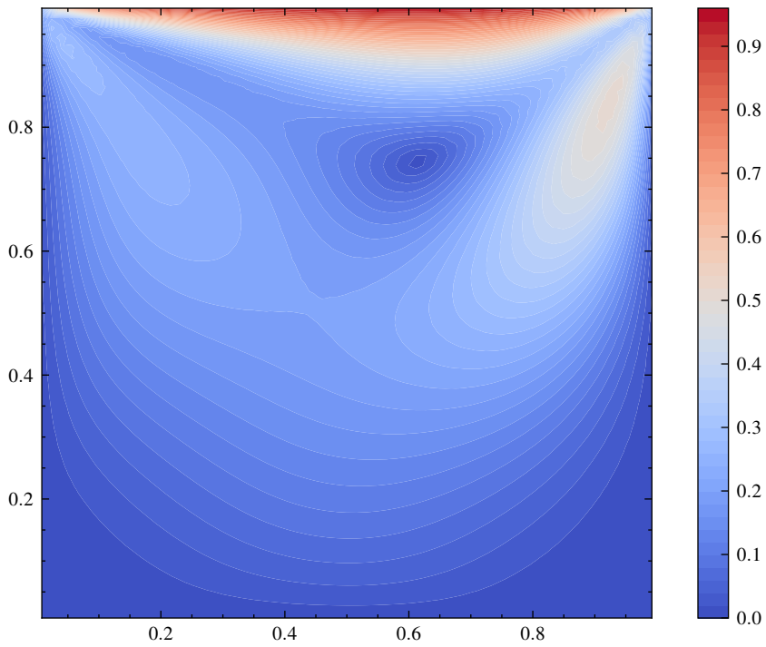
Velocity Magnitude
