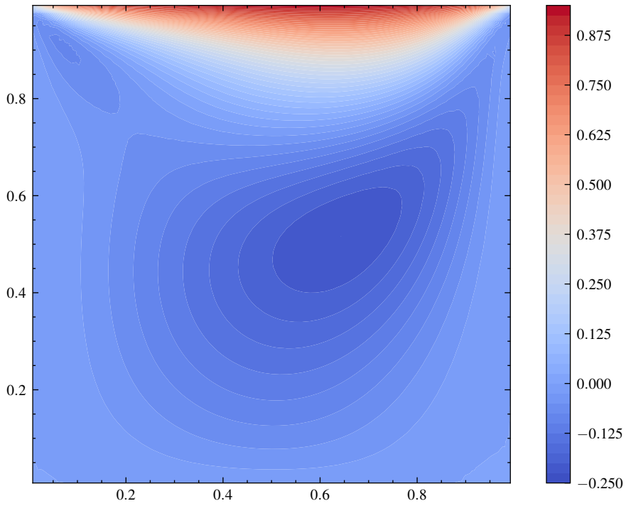
U-velocity
