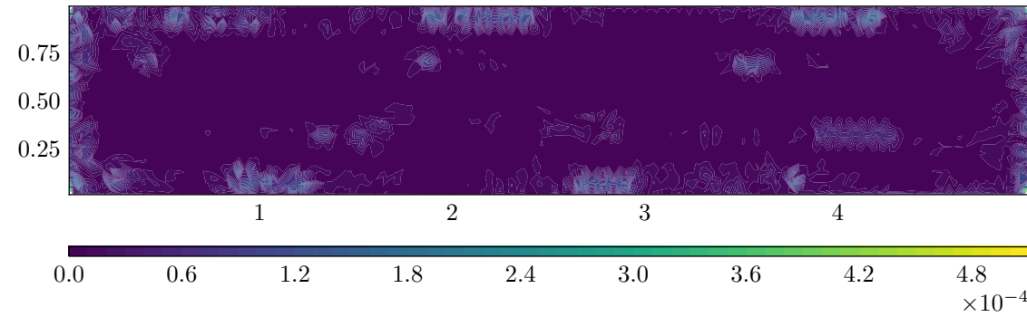
Continuity Residual
