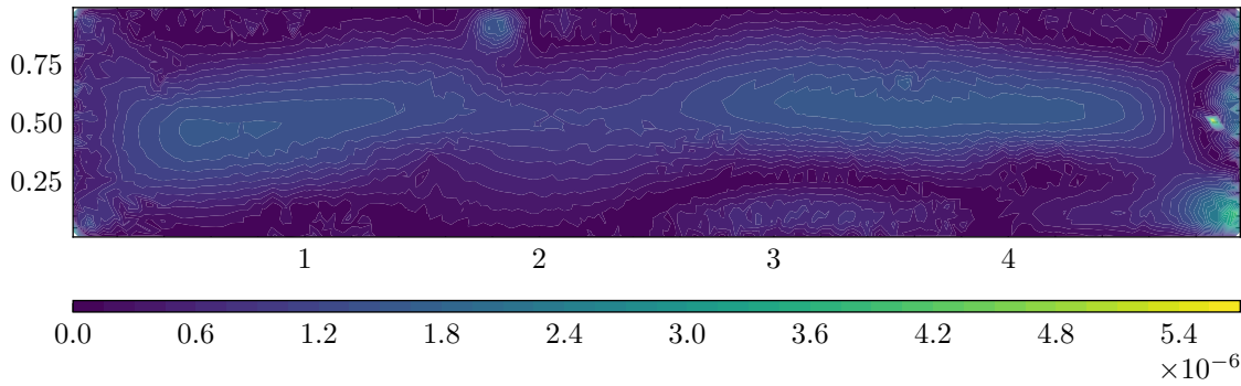
U Residual
