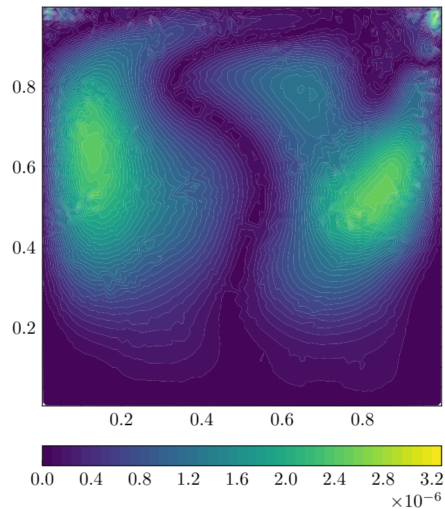
V Residual
