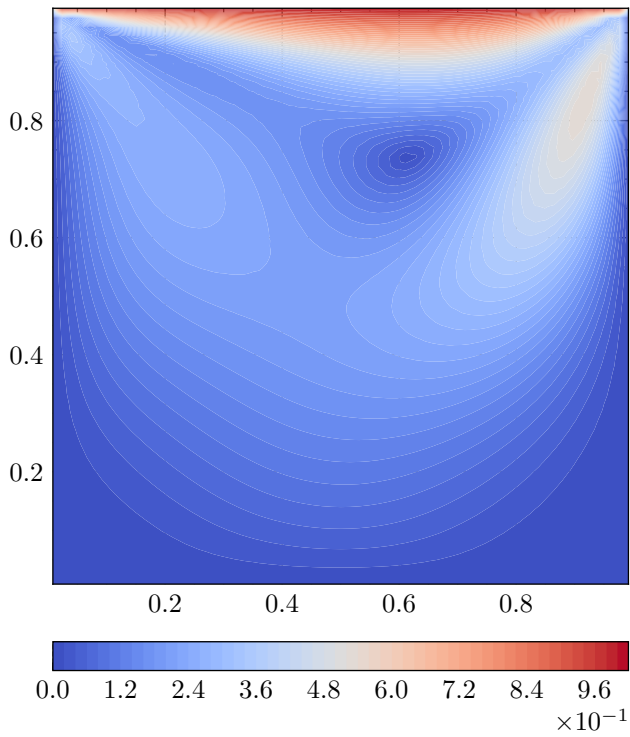
Velocity Magnitude
