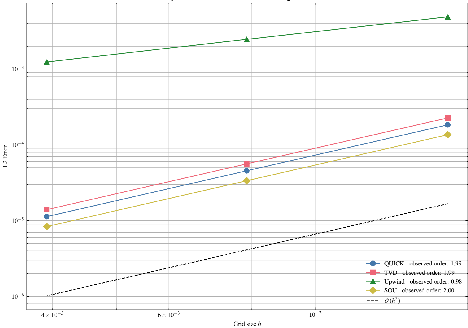
Order of Accuracy Convection-Diffusion Equation - Structured Mesh
