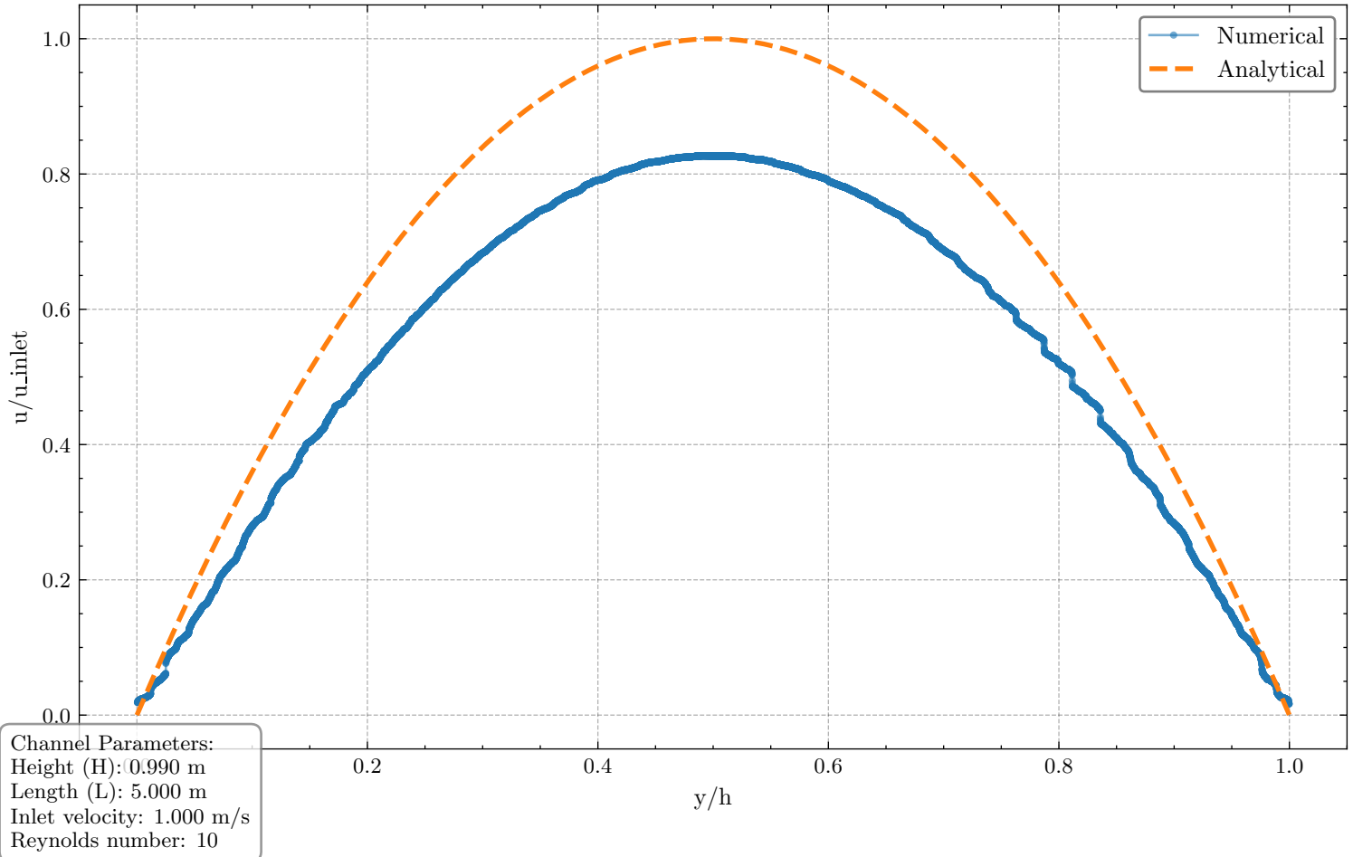
Velocity Profile at x=L/2
