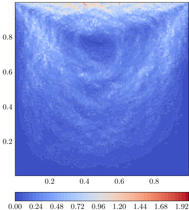
Velocity Magnitude
