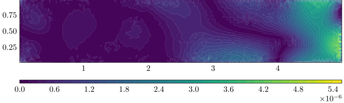
V Residual
