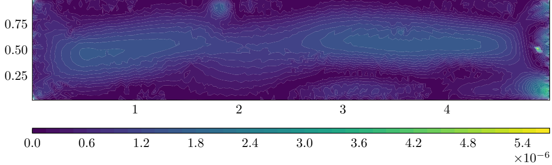
U Residual
