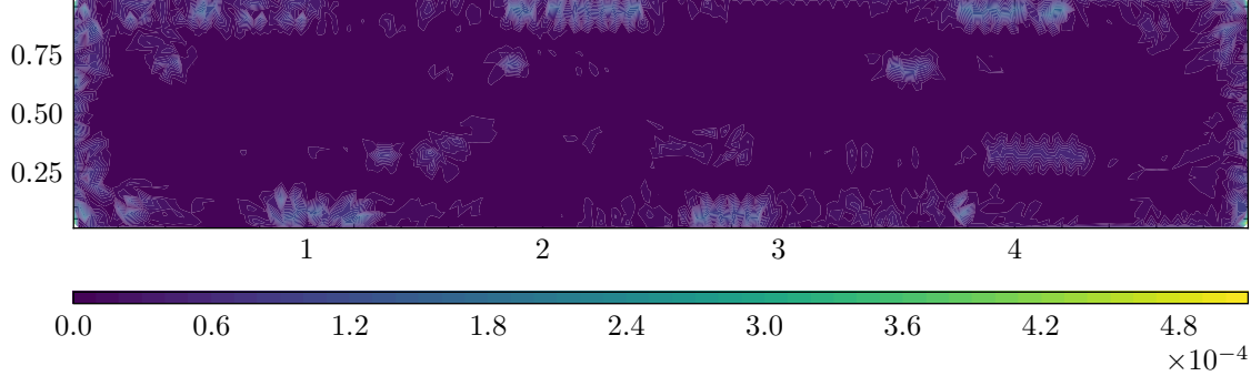
Continuity Residual
