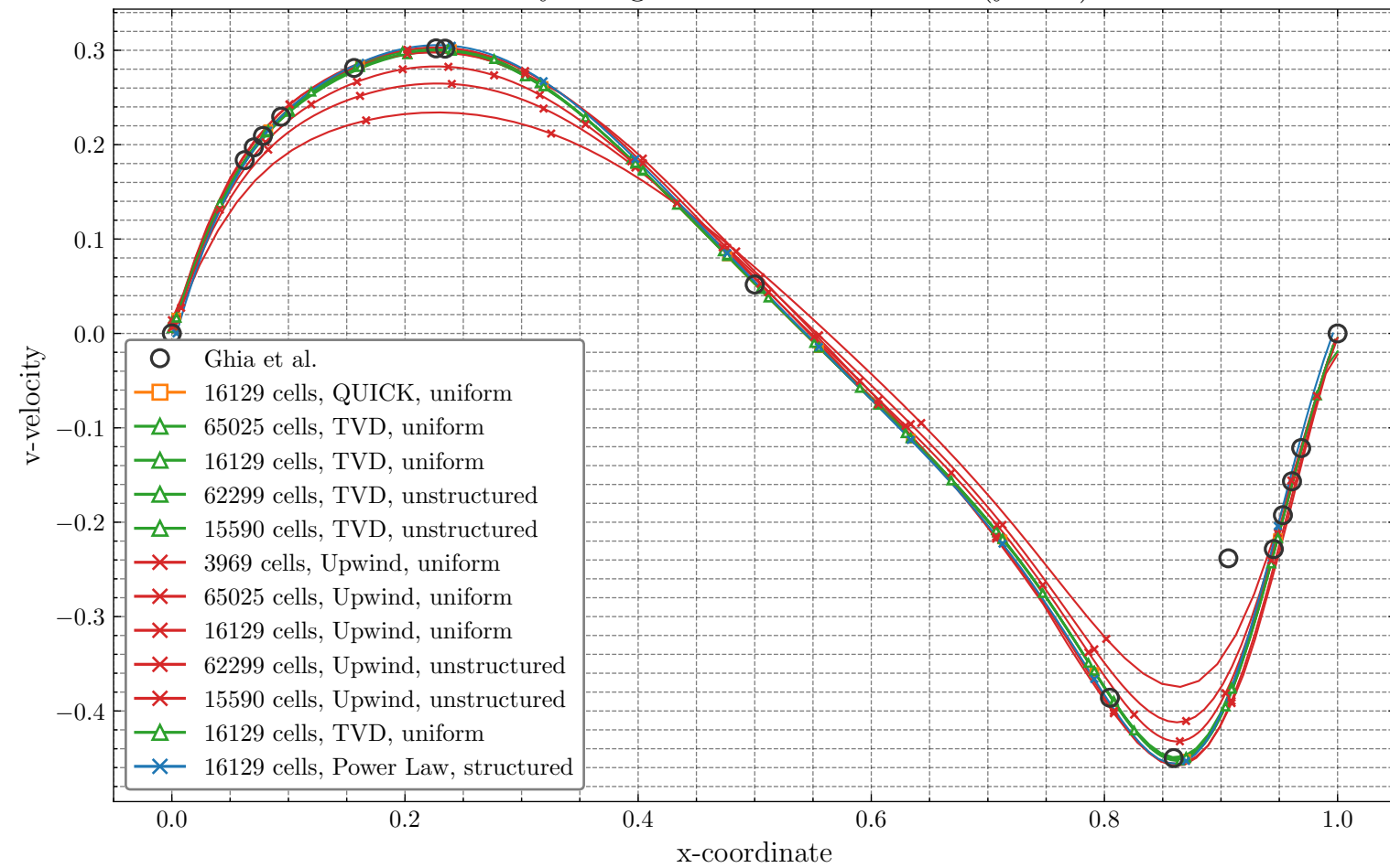
v-velocity along Horizontal Centerline (y=0.5)
