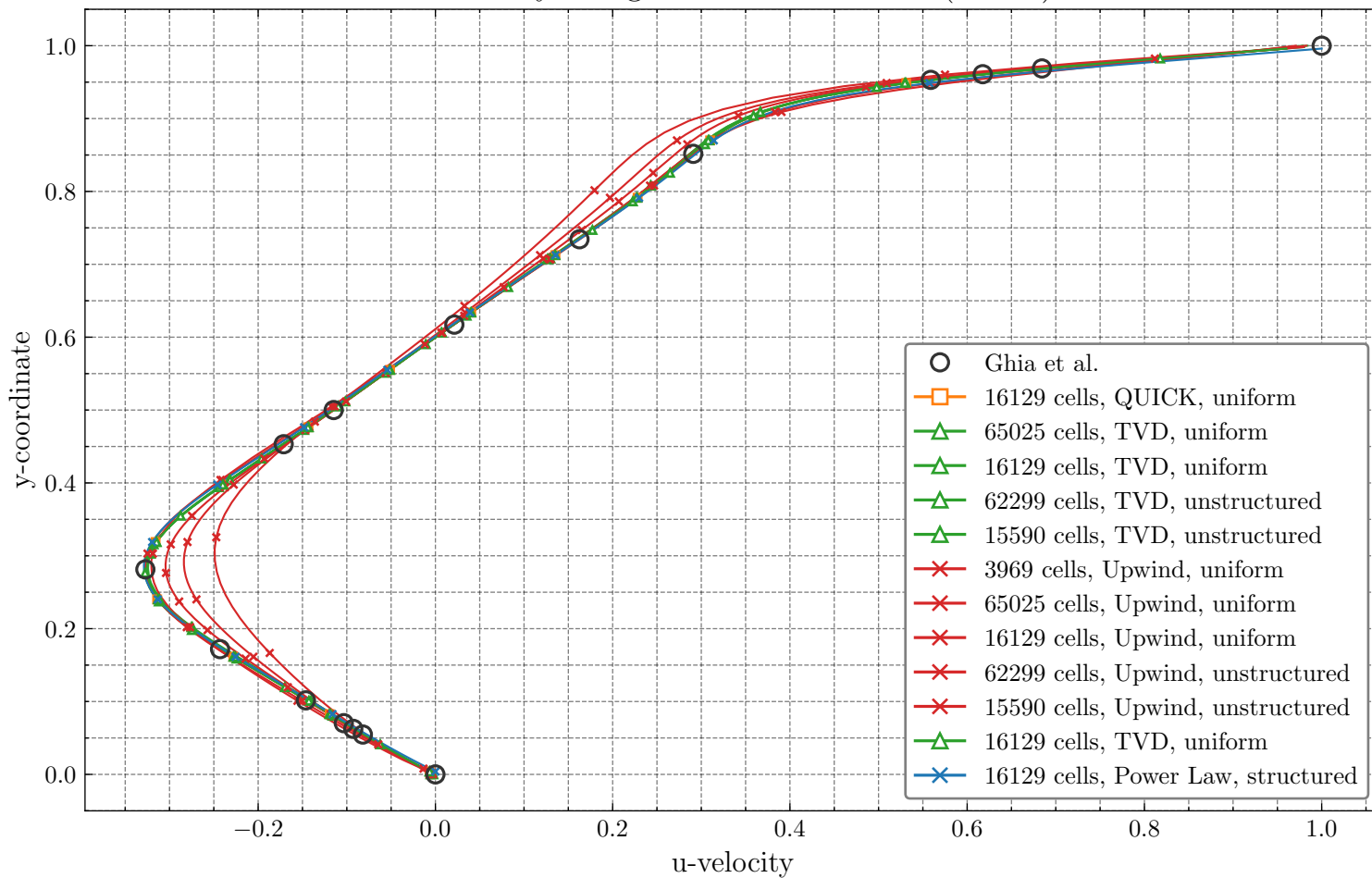
u-velocity along Vertical Centerline (x=0.5)
