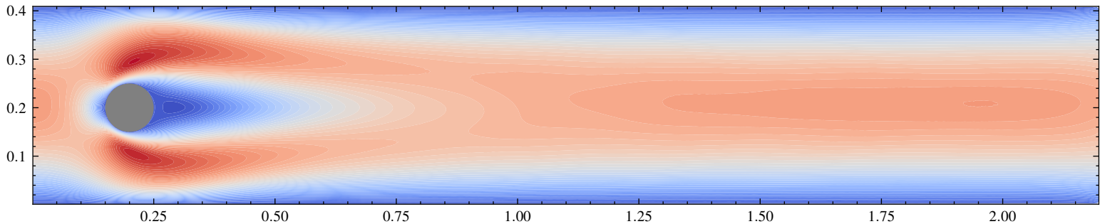
u-velocity — Simulation ID: de9cadff
