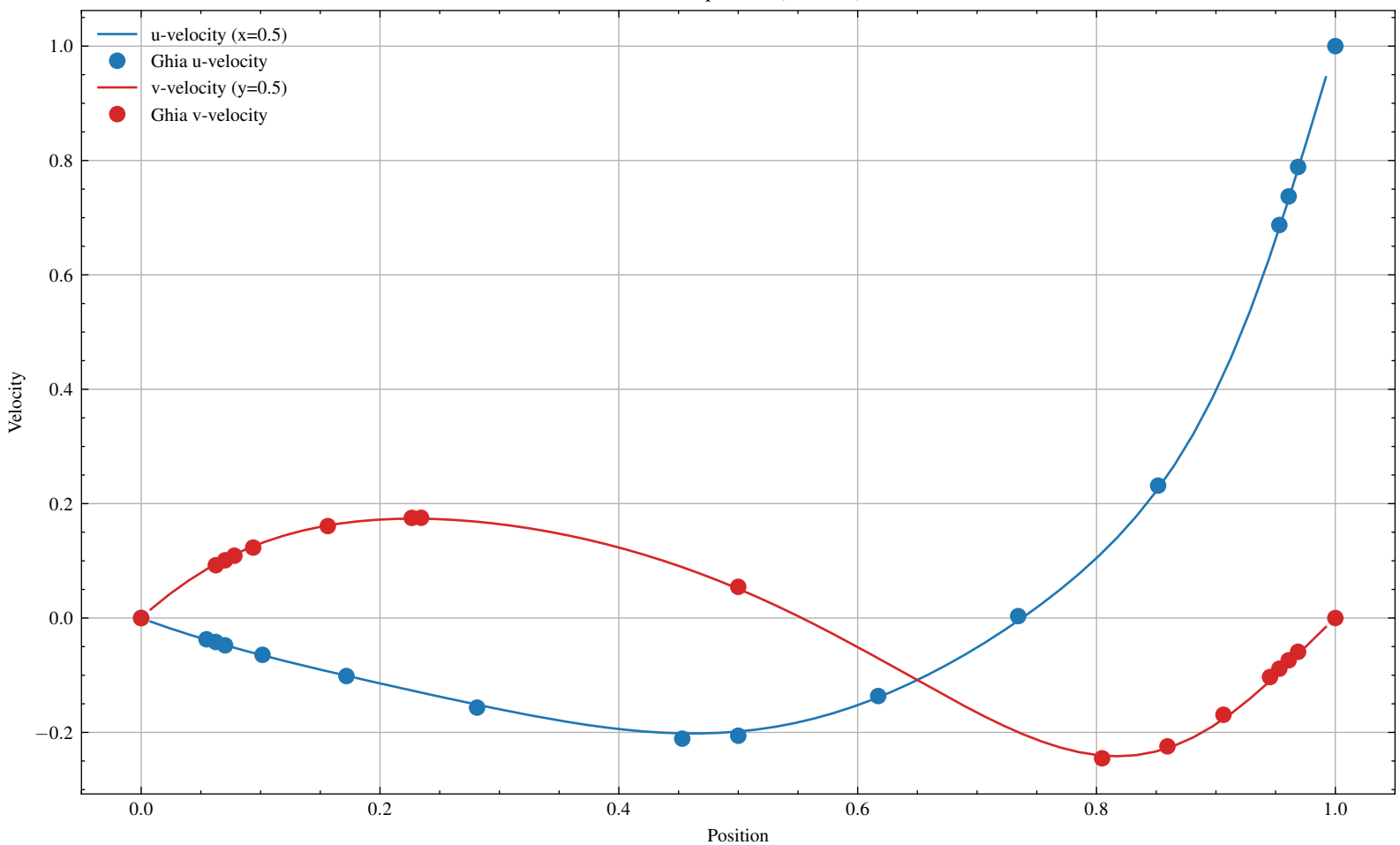
Ghia Comparison (Re=100)
