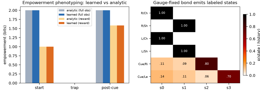
Fig. 7. Left: empowerment phenotyping on the learned full-maze model matches analytic across the zero-, intermediate-, and maximal-control regimes, full-observation and reward-only. Right: the gauge-fixed bond emits labelled states (minimal maze); trap histories are near one-hot, cue histories softer.
