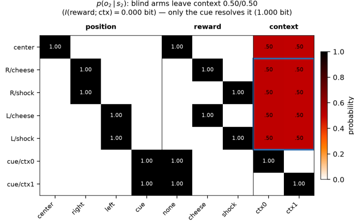
Fig. 4. Emission p(o_2 | s_2) of the learned full-maze model, factored into Position, Reward, and Context. The four arm states (boxed) are separated by their reward but leave context at 0.50/0.50: a blind arm carries I(\text{reward}; \text{context}) = 0 bits, so it resolves no hidden state. Only the two cue states fix the context, where the read-off bit is worth 1 bit about the next arm’s reward.
