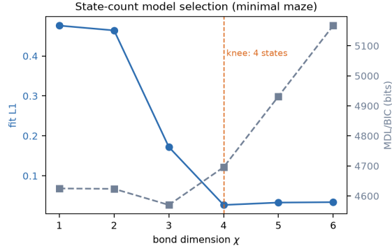
Fig. 6. State-count selection (minimal maze). Fit L1 (blue) drops \sim 6\times from \chi = 3 to \chi = 4 and then plateaus; bond dimension beyond four is spare capacity. The description-length score (grey) is one state more conservative.
