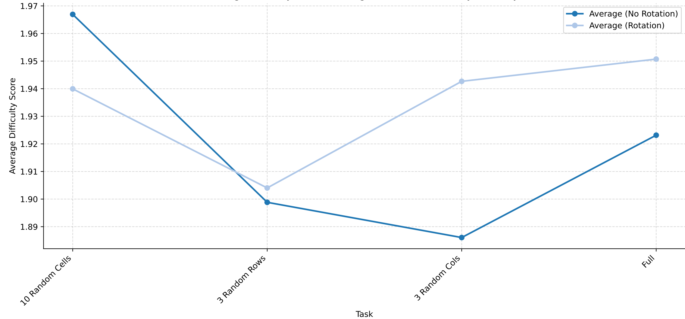
Average Difficulty Score - Average Across Models (Easy Difficulty)
