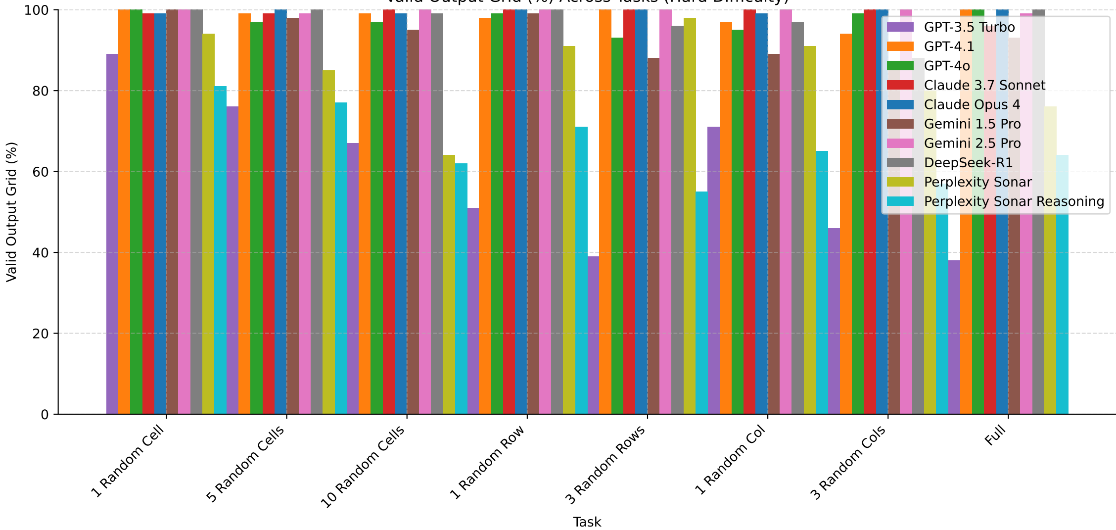
Valid Output Grid (%) Across Tasks (Hard Difficulty)
