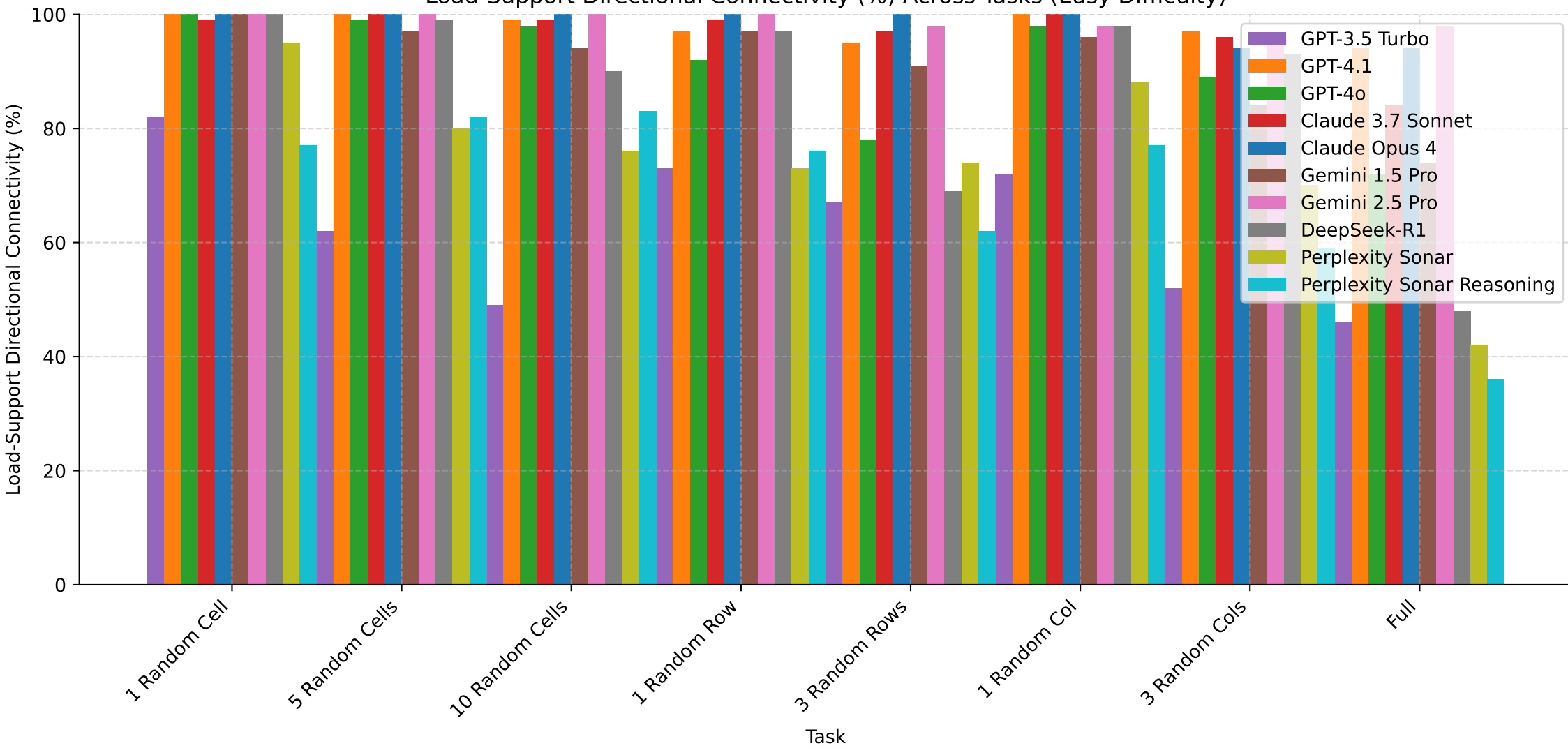
Load-Support Directional Connectivity (%) Across Tasks (Easy Difficulty)
