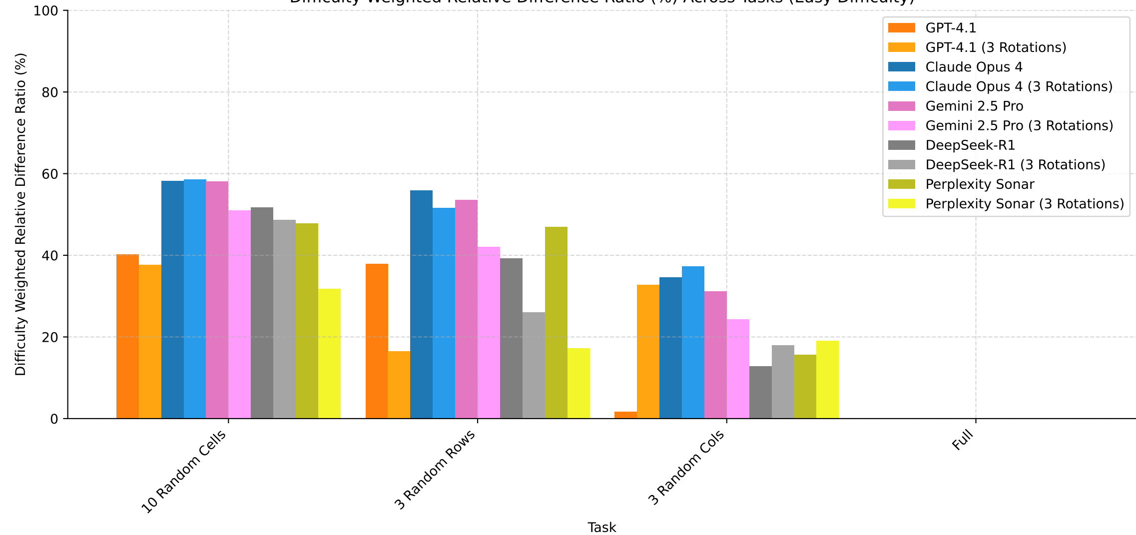
Difficulty Weighted Relative Difference Ratio (%) Across Tasks (Easy Difficulty)
