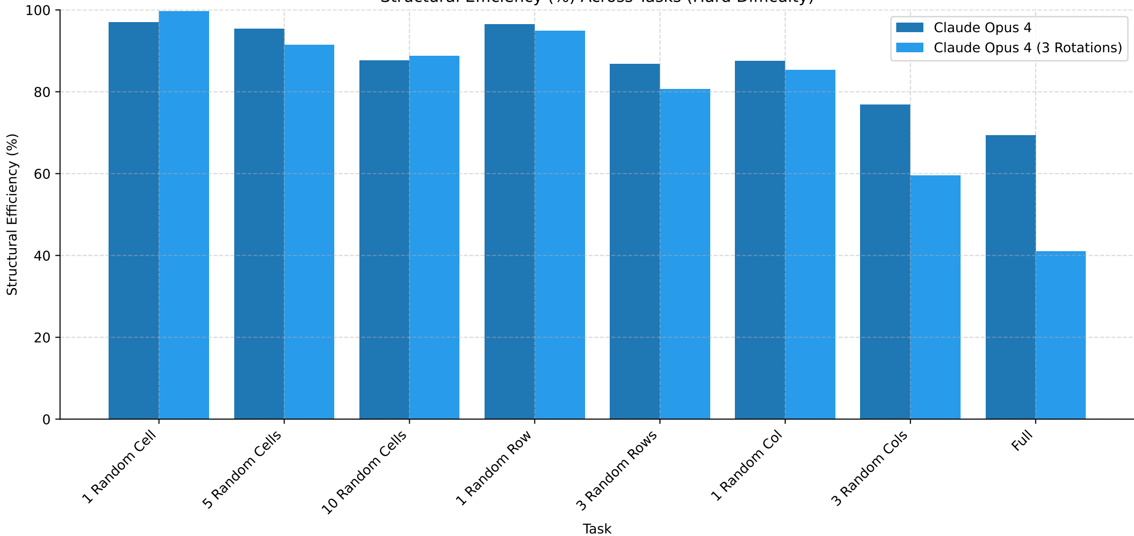
Structural Efficiency (%) Across Tasks (Hard Difficulty)
