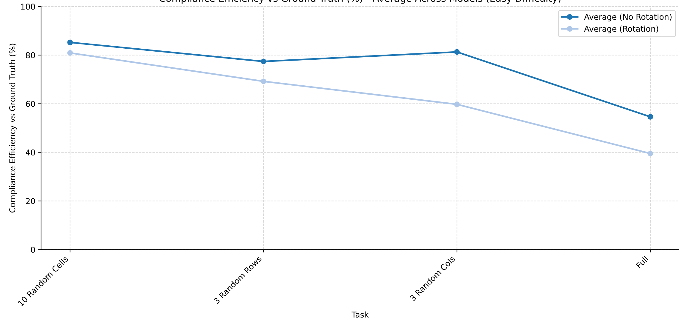
Compliance Efficiency vs Ground Truth (%) - Average Across Models (Easy Difficulty)
