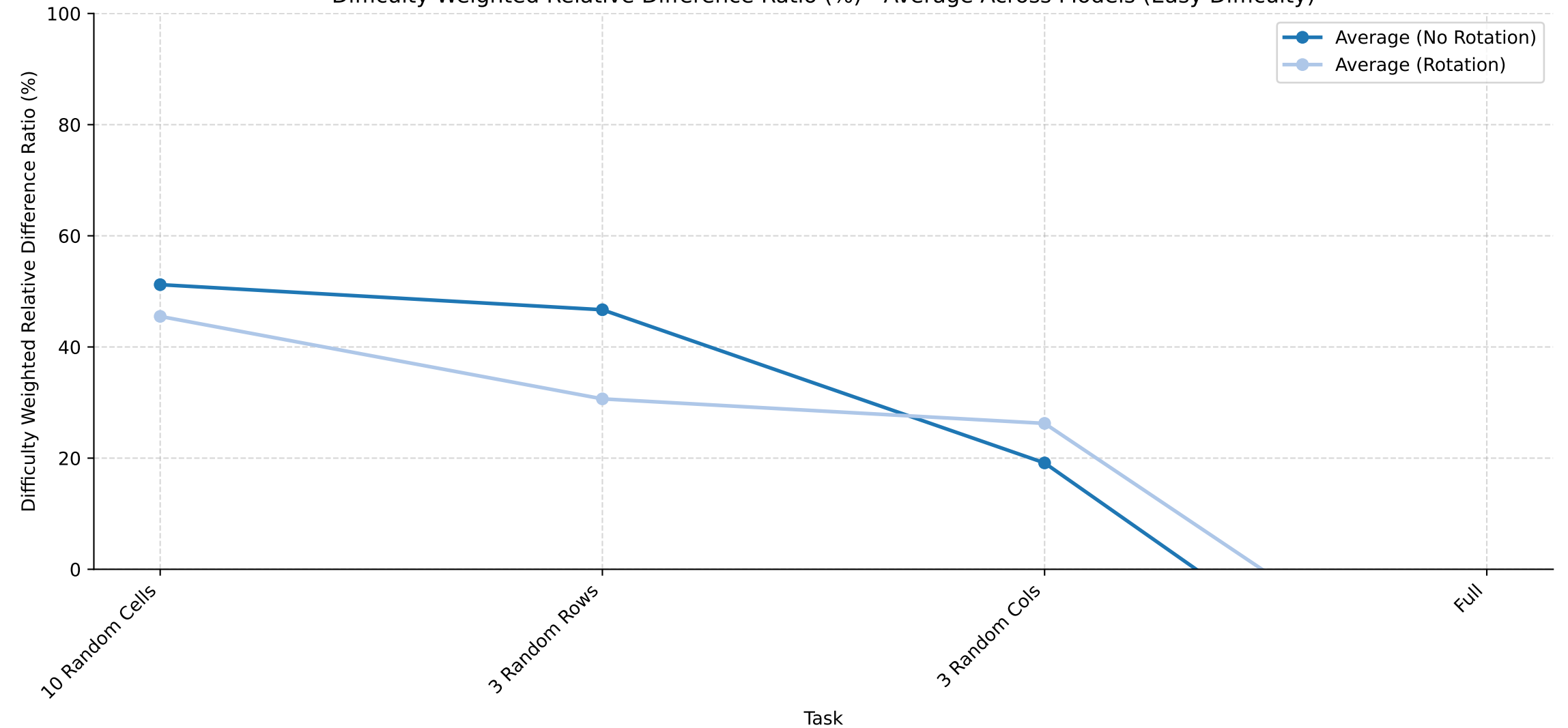
Difficulty Weighted Relative Difference Ratio (%) - Average Across Models (Easy Difficulty)
