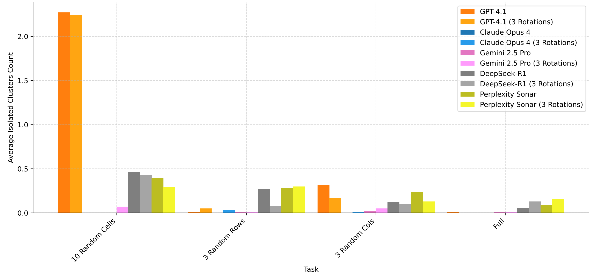
Average Isolated Clusters Count Across Tasks (Easy Difficulty)
