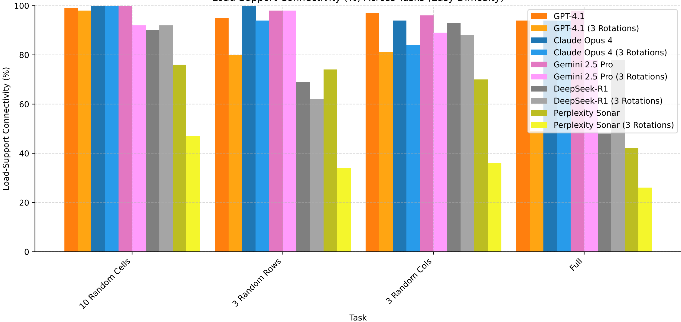
Load-Support Connectivity (%) Across Tasks (Easy Difficulty)
