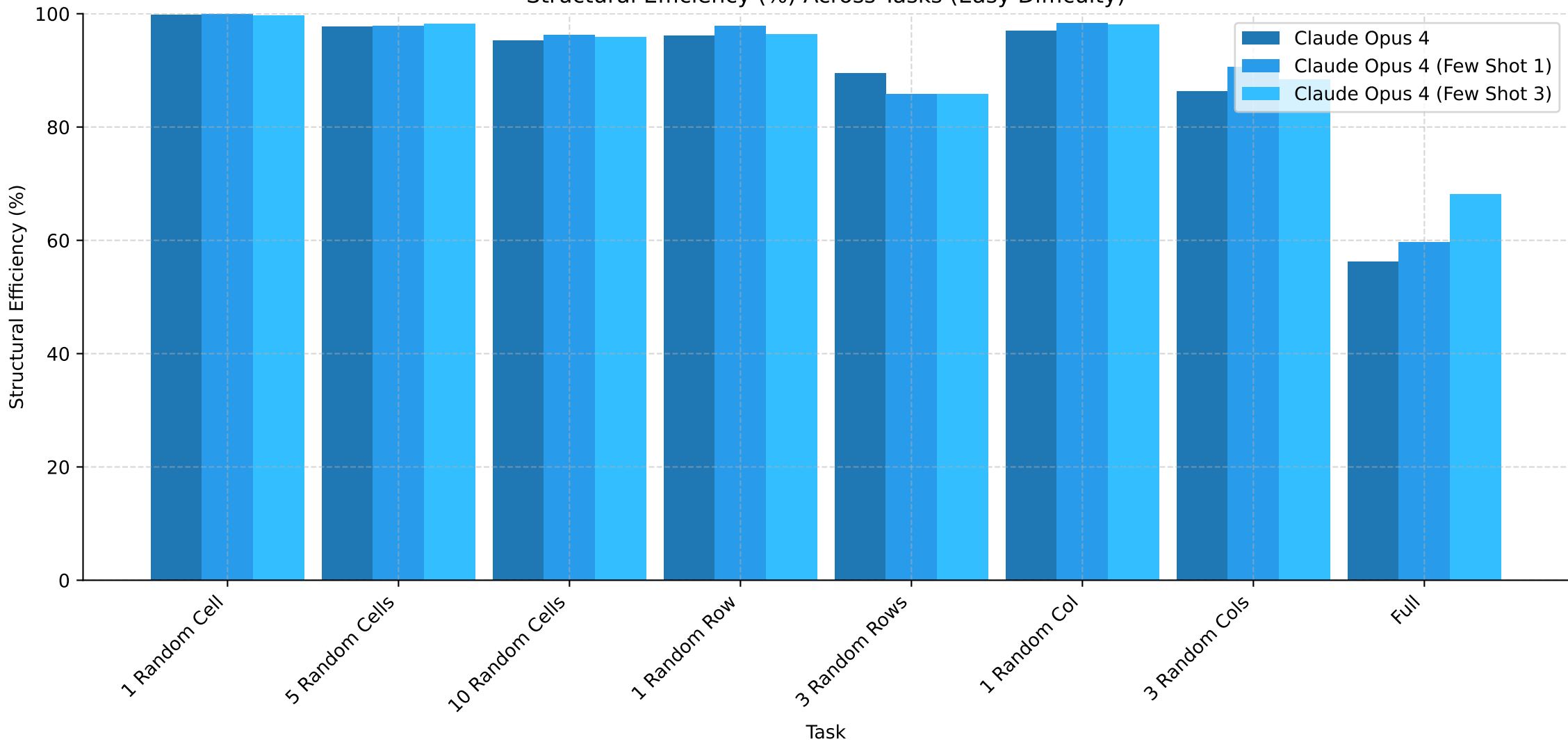
Structural Efficiency (%) Across Tasks (Easy Difficulty)
