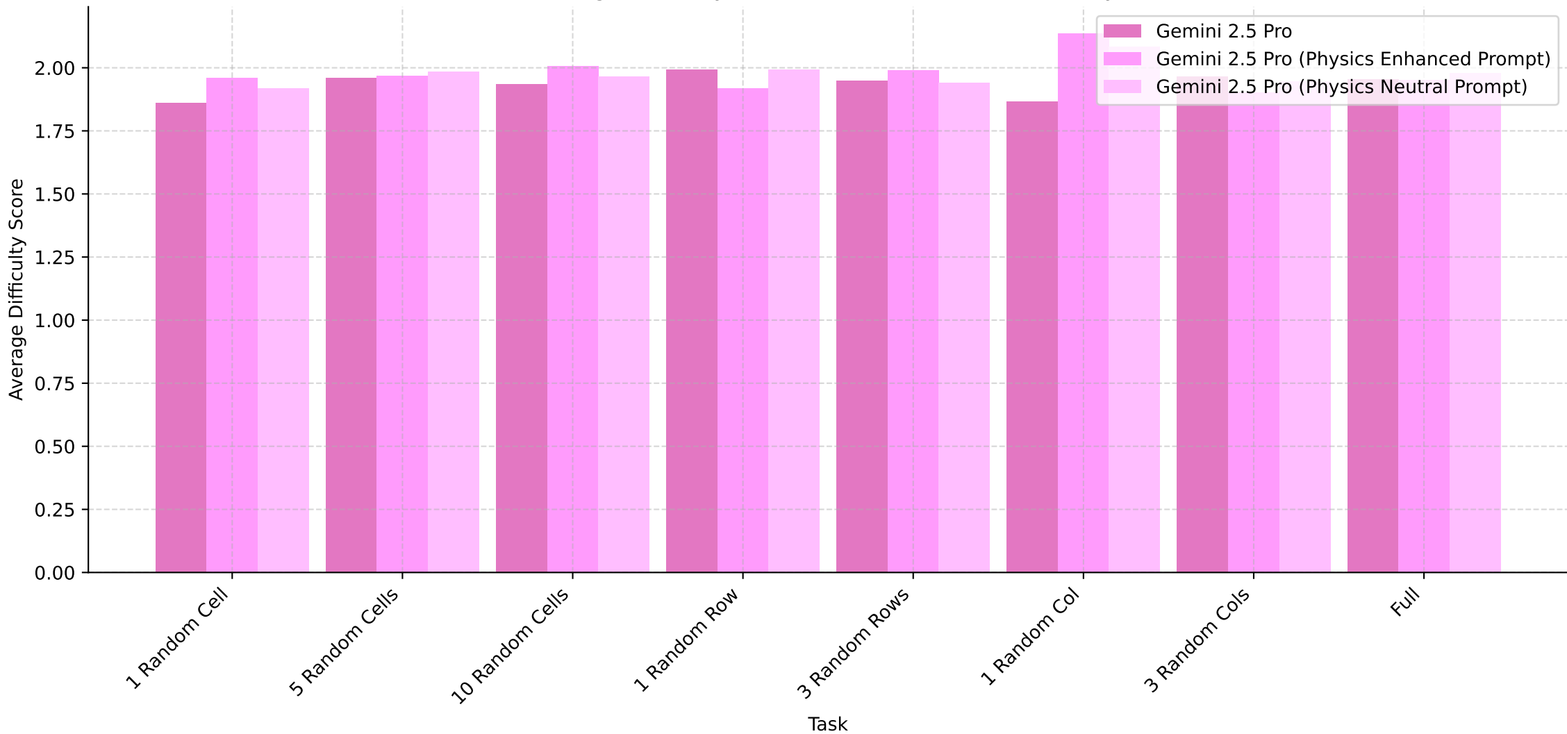
Average Difficulty Score Across Tasks (Hard Difficulty)
