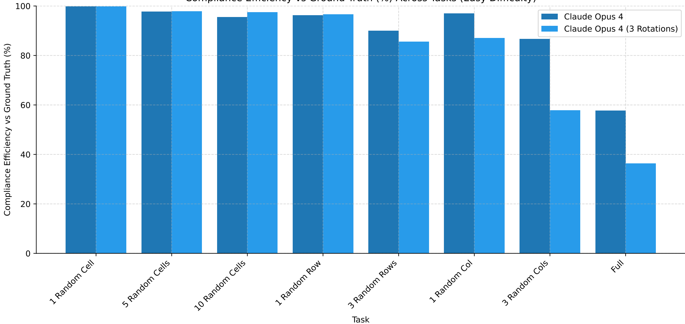
Compliance Efficiency vs Ground Truth (%) Across Tasks (Easy Difficulty)
