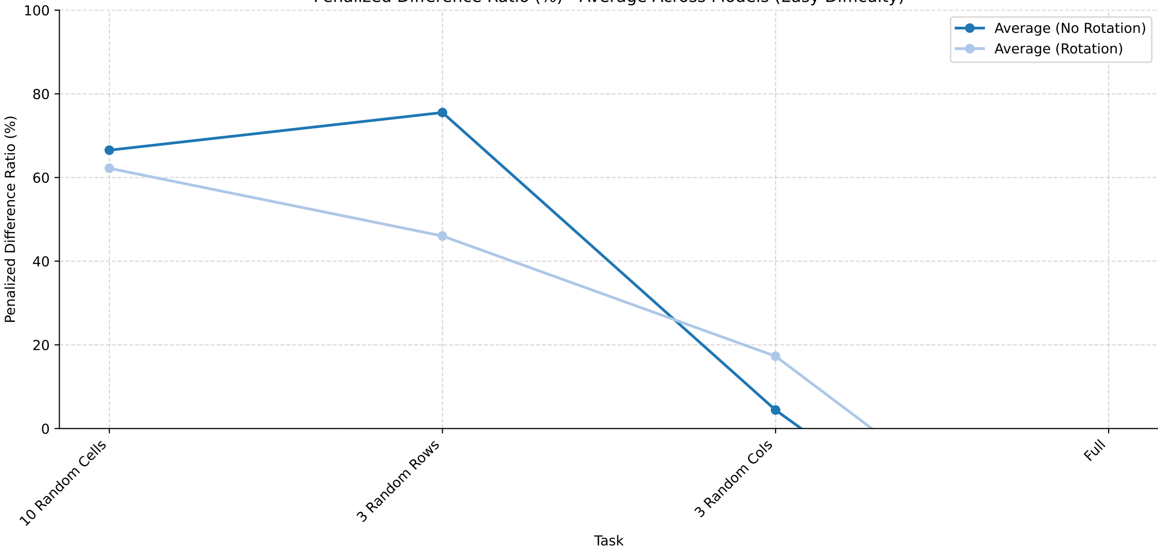
Penalized Difference Ratio (%) - Average Across Models (Easy Difficulty)
