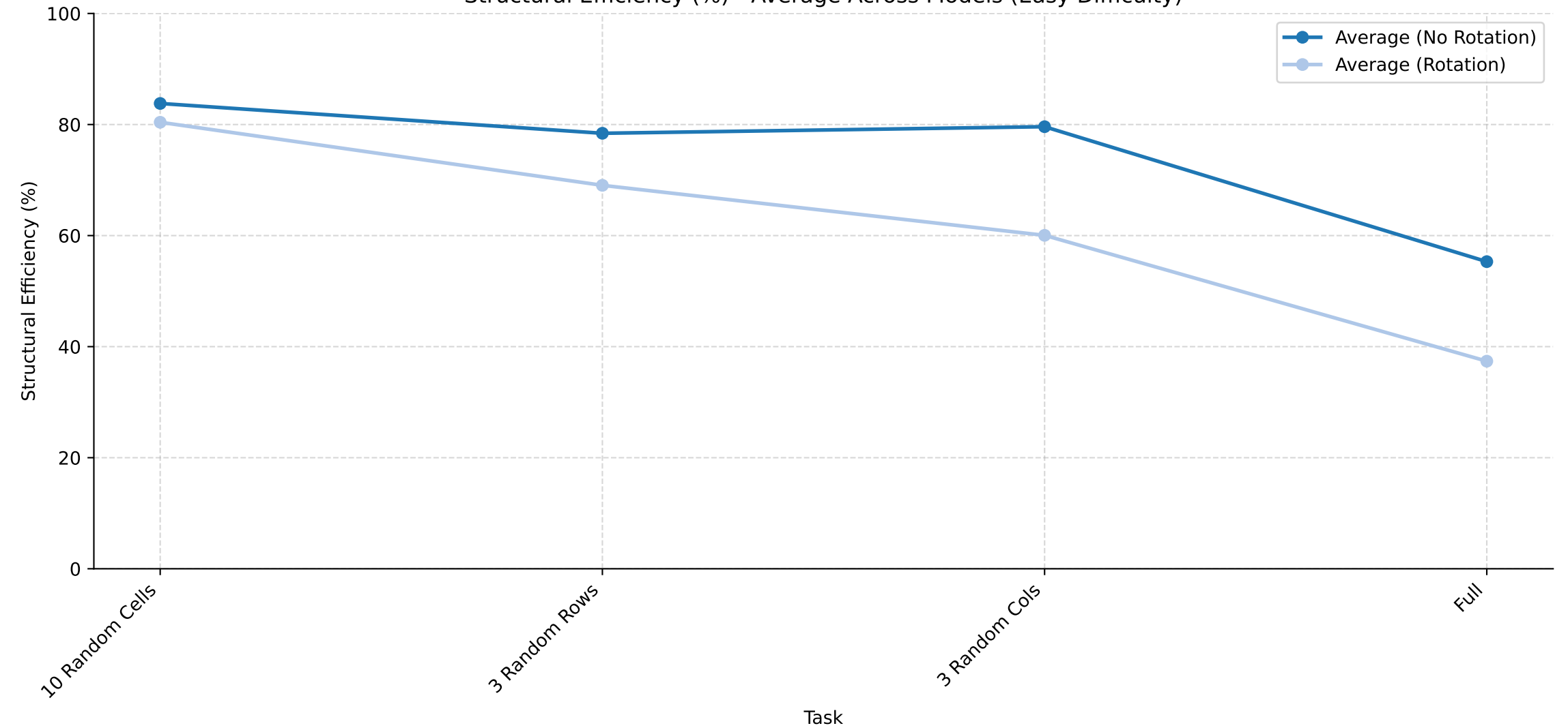
Structural Efficiency (%) - Average Across Models (Easy Difficulty)
