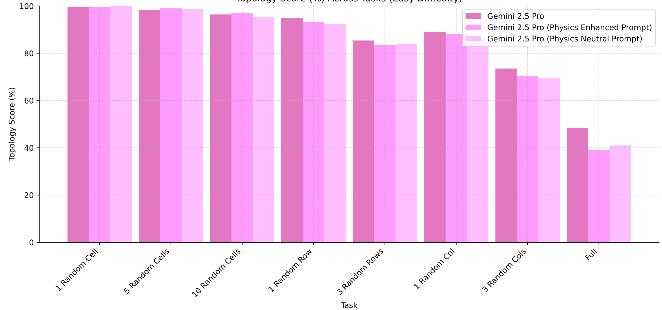
Topology Score (%) Across Tasks (Easy Difficulty)
